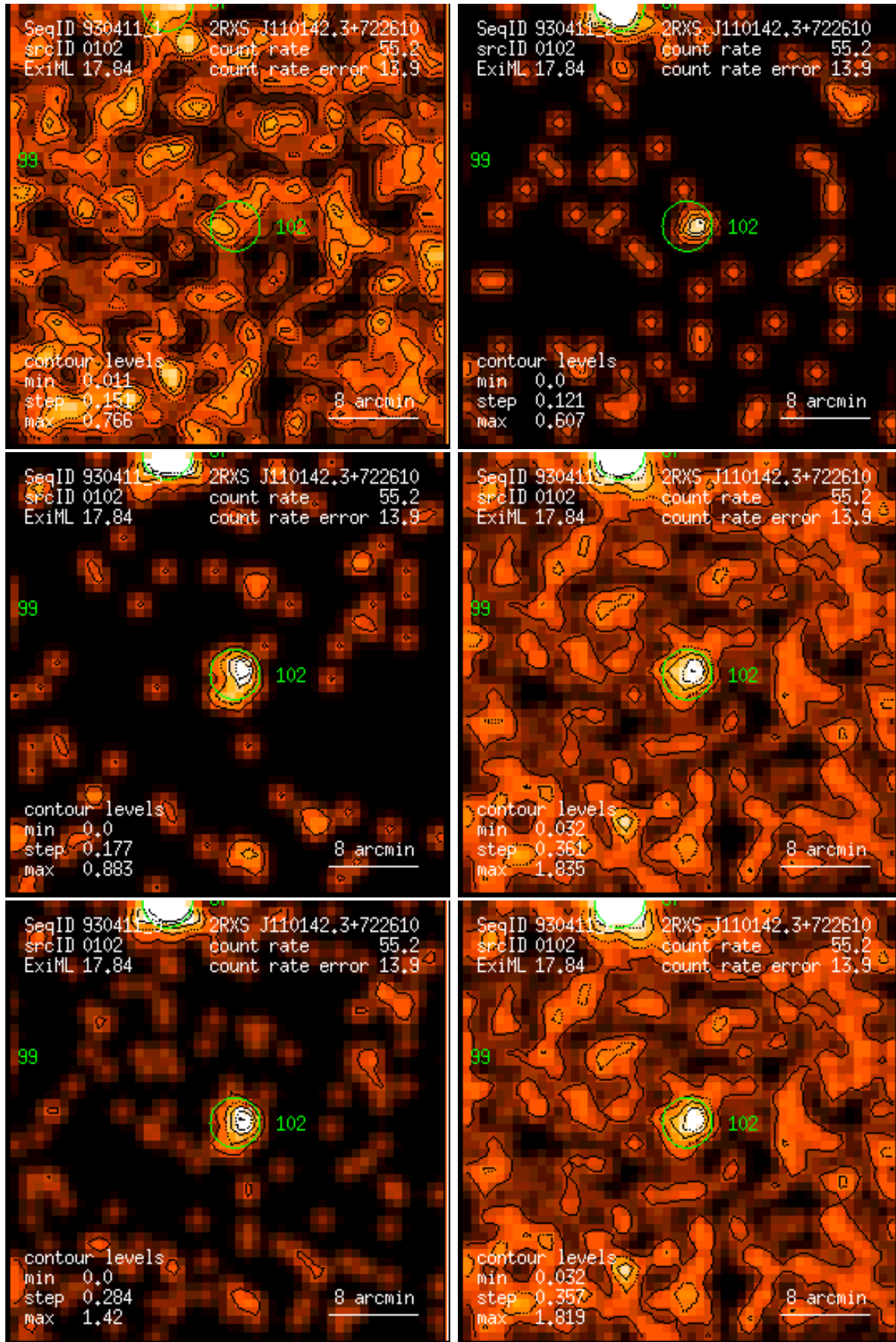
Figure 102: RASS 930411: detection 0102: band rate images, Gaussian filter: (1) PSPC channels 11 – 41, (2) 52 – 90, (3) 91 – 201, (4) 11 – 235, (5) 52 – 201, (6) 11 – 201. Broad band rates in counts/ks. Band rate contour levels in counts/ks/arcmin 2 .
