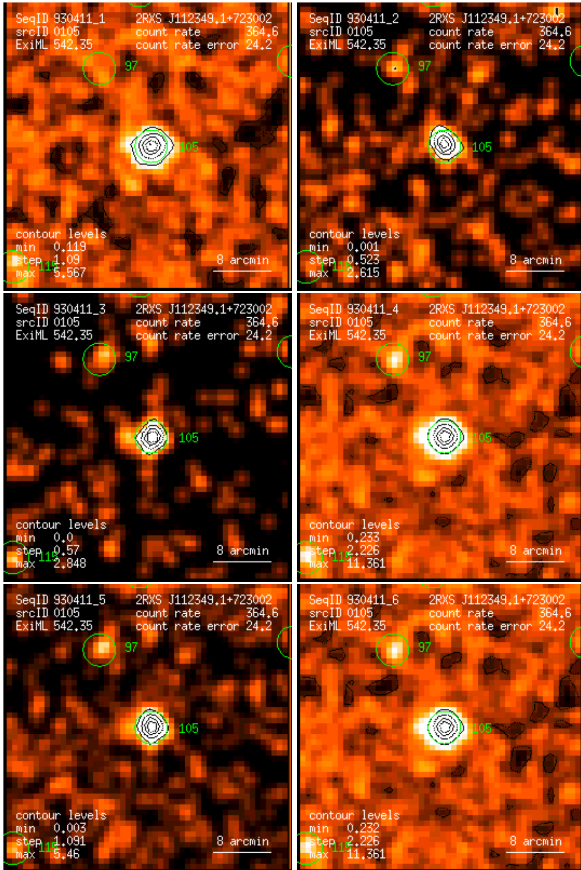
Figure 105: RASS 930411: detection 0105: band rate images, Gaussian filter: (1) PSPC channels 11 – 41, (2) 52 – 90, (3) 91 – 201, (4) 11 – 235, (5) 52 – 201, (6) 11 – 201. Broad band rates in counts/ks. Band rate contour levels in counts/ks/arcmin 2 .
