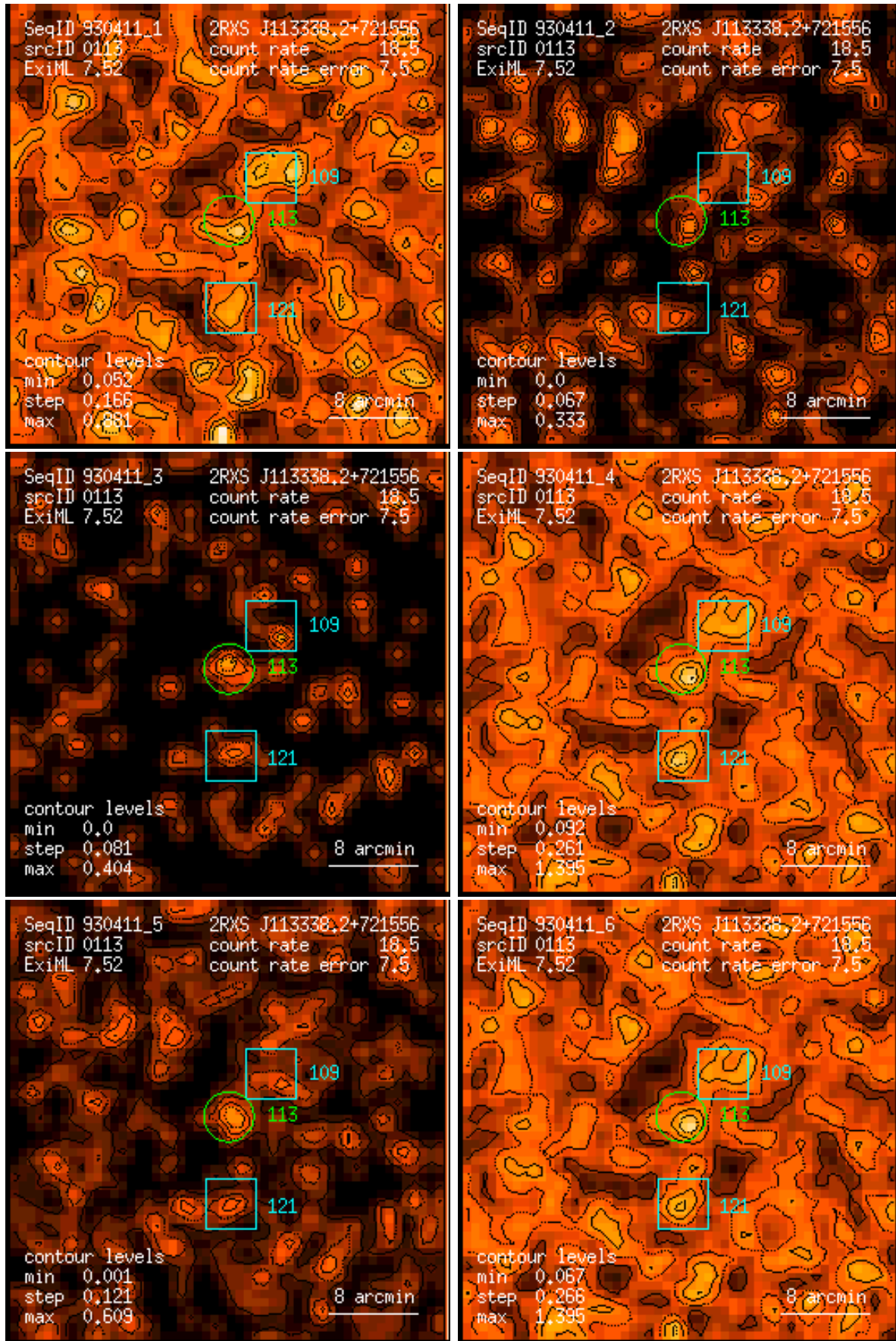
Figure 113: RASS 930411: detection 0113: band rate images, Gaussian filter: (1) PSPC channels 11 – 41, (2) 52 – 90, (3) 91 – 201, (4) 11 – 235, (5) 52 – 201, (6) 11 – 201. Broad band rates in counts/ks. Band rate contour levels in counts/ks/arcmin 2 .
