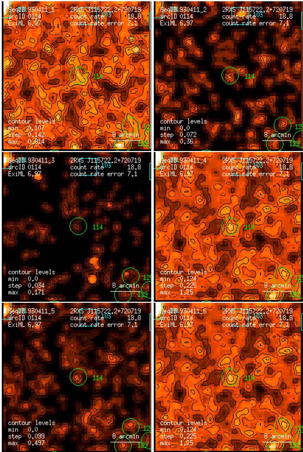
Figure 114: RASS 930411: detection 0114: band rate images, Gaussian filter: (1) PSPC channels 11 – 41, (2) 52 – 90, (3) 91 – 201, (4) 11 – 235, (5) 52 – 201, (6) 11 – 201. Broad band rates in counts/ks. Band rate contour levels in counts/ks/arcmin 2 .
