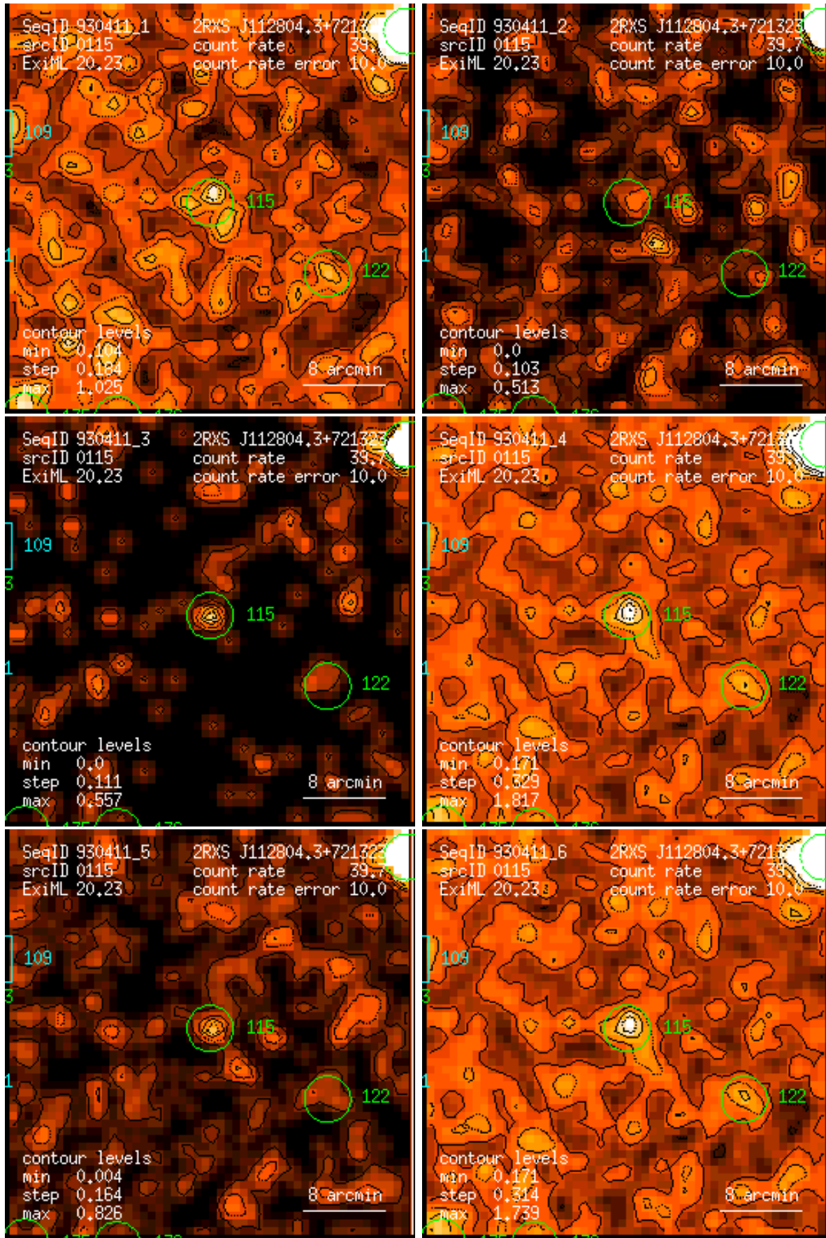
Figure 115: RASS 930411: detection 0115: band rate images, Gaussian filter: (1) PSPC channels 11 – 41, (2) 52 – 90, (3) 91 – 201, (4) 11 – 235, (5) 52 – 201, (6) 11 – 201. Broad band rates in counts/ks. Band rate contour levels in counts/ks/arcmin 2 .
