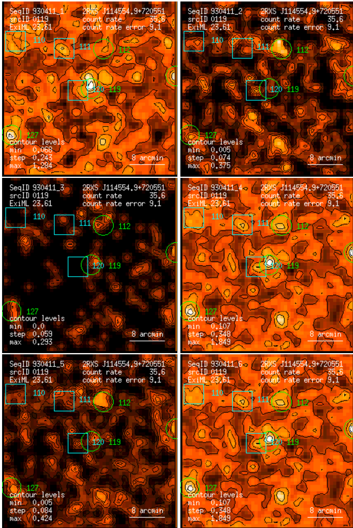
Figure 119: RASS 930411: detection 0119: band rate images, Gaussian filter: (1) PSPC channels 11 – 41, (2) 52 – 90, (3) 91 – 201, (4) 11 – 235, (5) 52 – 201, (6) 11 – 201. Broad band rates in counts/ks. Band rate contour levels in counts/ks/arcmin 2 .
