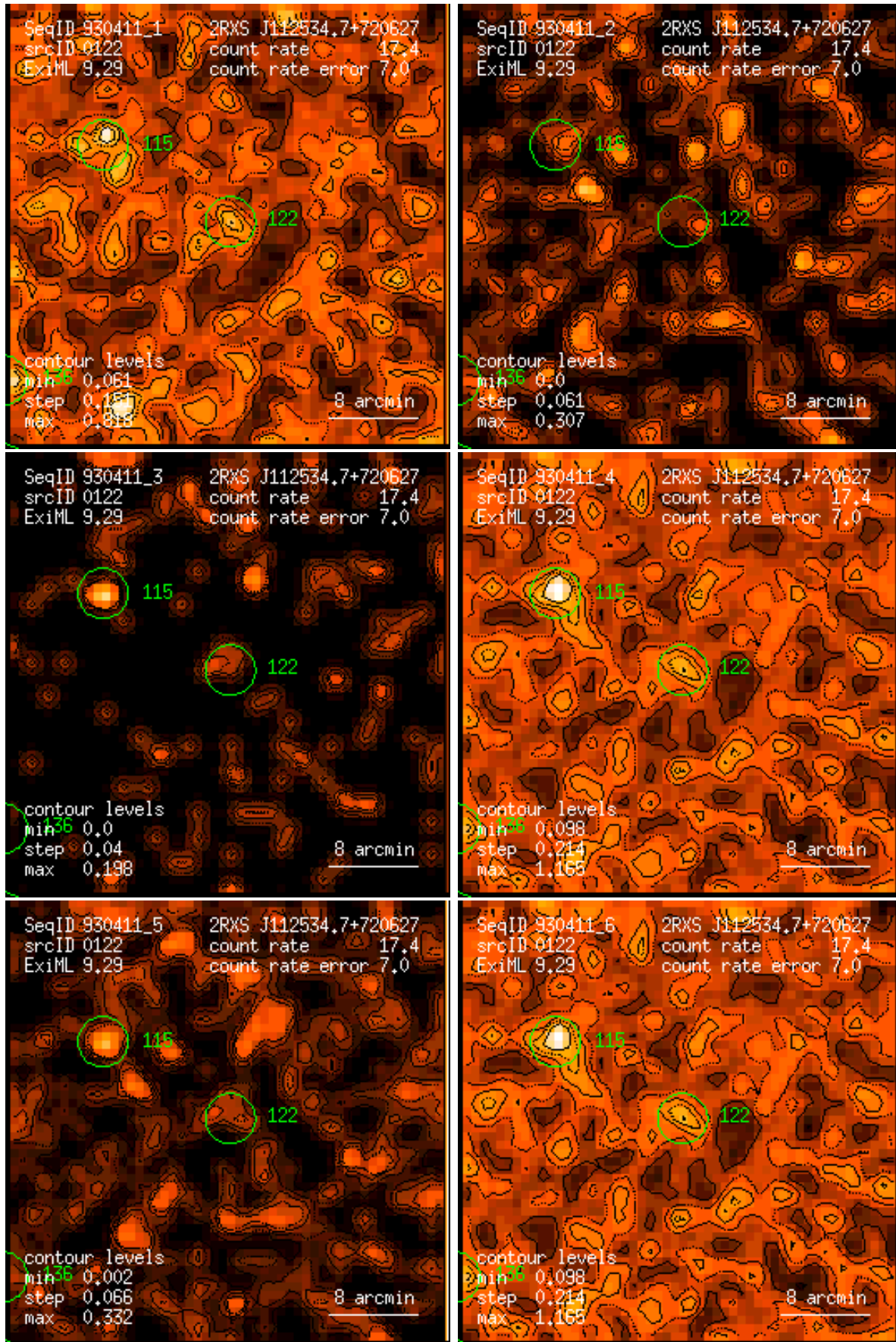
Figure 122: RASS 930411: detection 0122: band rate images, Gaussian filter: (1) PSPC channels 11 – 41, (2) 52 – 90, (3) 91 – 201, (4) 11 – 235, (5) 52 – 201, (6) 11 – 201. Broad band rates in counts/ks. Band rate contour levels in counts/ks/arcmin 2 .
