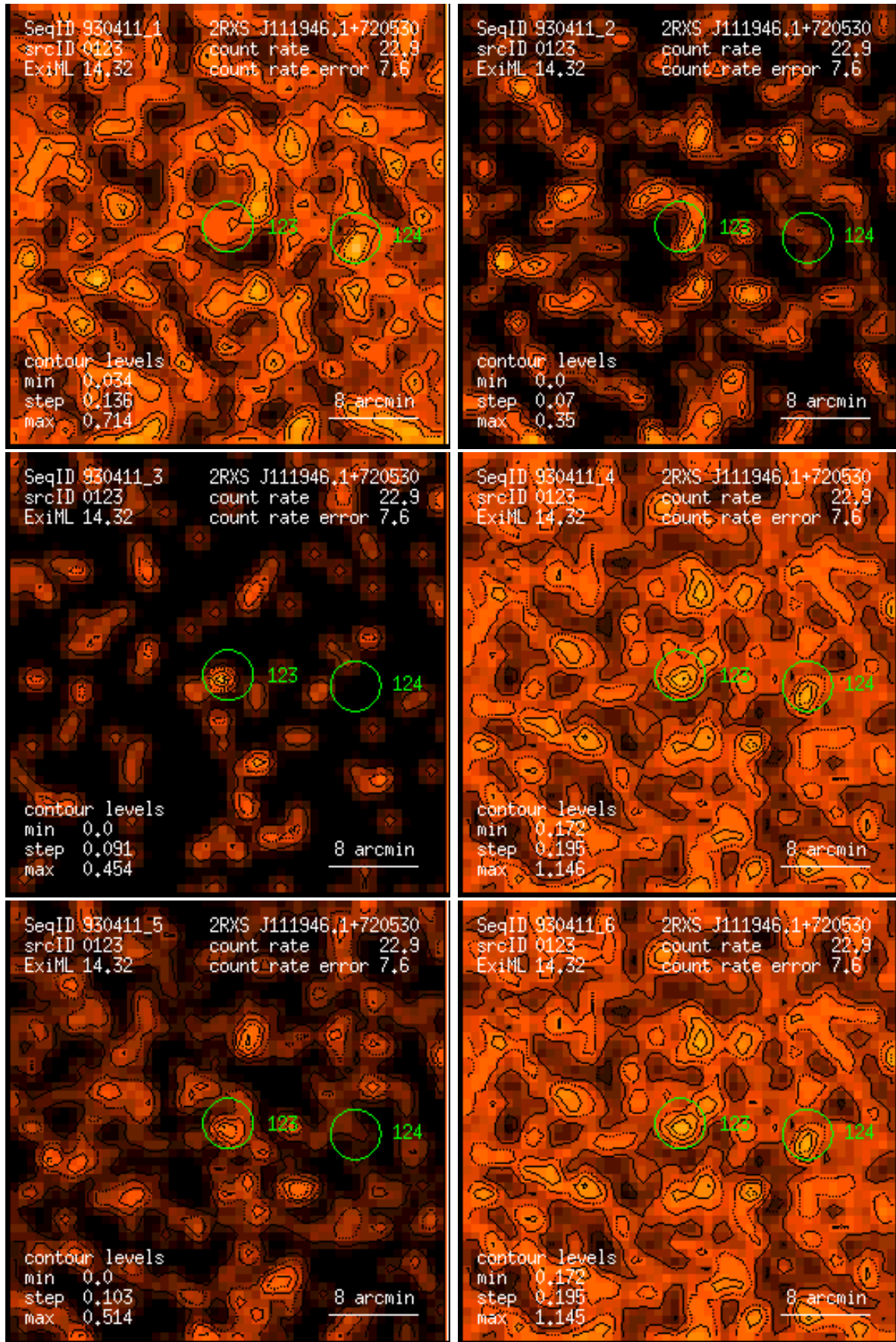
Figure 123: RASS 930411: detection 0123: band rate images, Gaussian filter: (1) PSPC channels 11 – 41, (2) 52 – 90, (3) 91 – 201, (4) 11 – 235, (5) 52 – 201, (6) 11 – 201. Broad band rates in counts/ks. Band rate contour levels in counts/ks/arcmin 2 .
