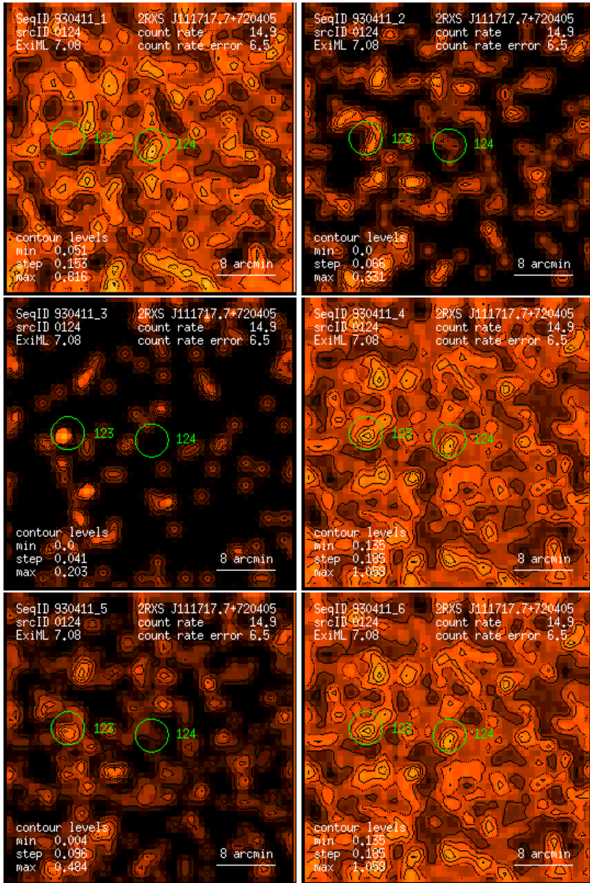
Figure 124: RASS 930411: detection 0124: band rate images, Gaussian filter: (1) PSPC channels 11 – 41, (2) 52 – 90, (3) 91 – 201, (4) 11 – 235, (5) 52 – 201, (6) 11 – 201. Broad band rates in counts/ks. Band rate contour levels in counts/ks/arcmin 2 .
