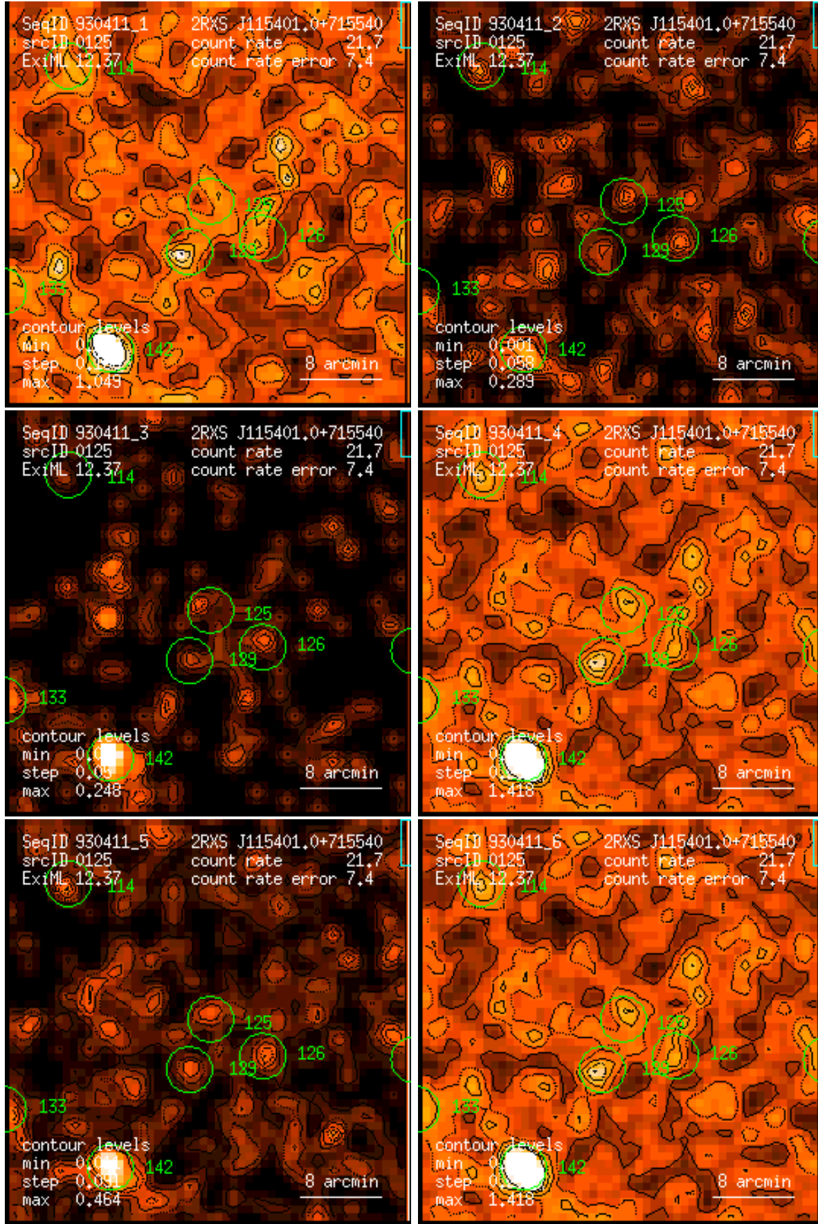
Figure 125: RASS 930411: detection 0125: band rate images, Gaussian filter: (1) PSPC channels 11 – 41, (2) 52 – 90, (3) 91 – 201, (4) 11 – 235, (5) 52 – 201, (6) 11 – 201. Broad band rates in counts/ks. Band rate contour levels in counts/ks/arcmin 2 .
