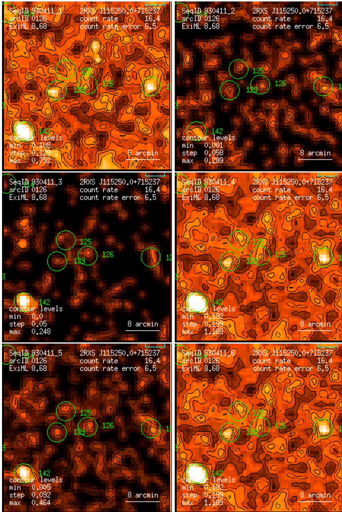
Figure 126: RASS 930411: detection 0126: band rate images, Gaussian filter: (1) PSPC channels 11 – 41, (2) 52 – 90, (3) 91 – 201, (4) 11 – 235, (5) 52 – 201, (6) 11 – 201. Broad band rates in counts/ks. Band rate contour levels in counts/ks/arcmin 2 .
