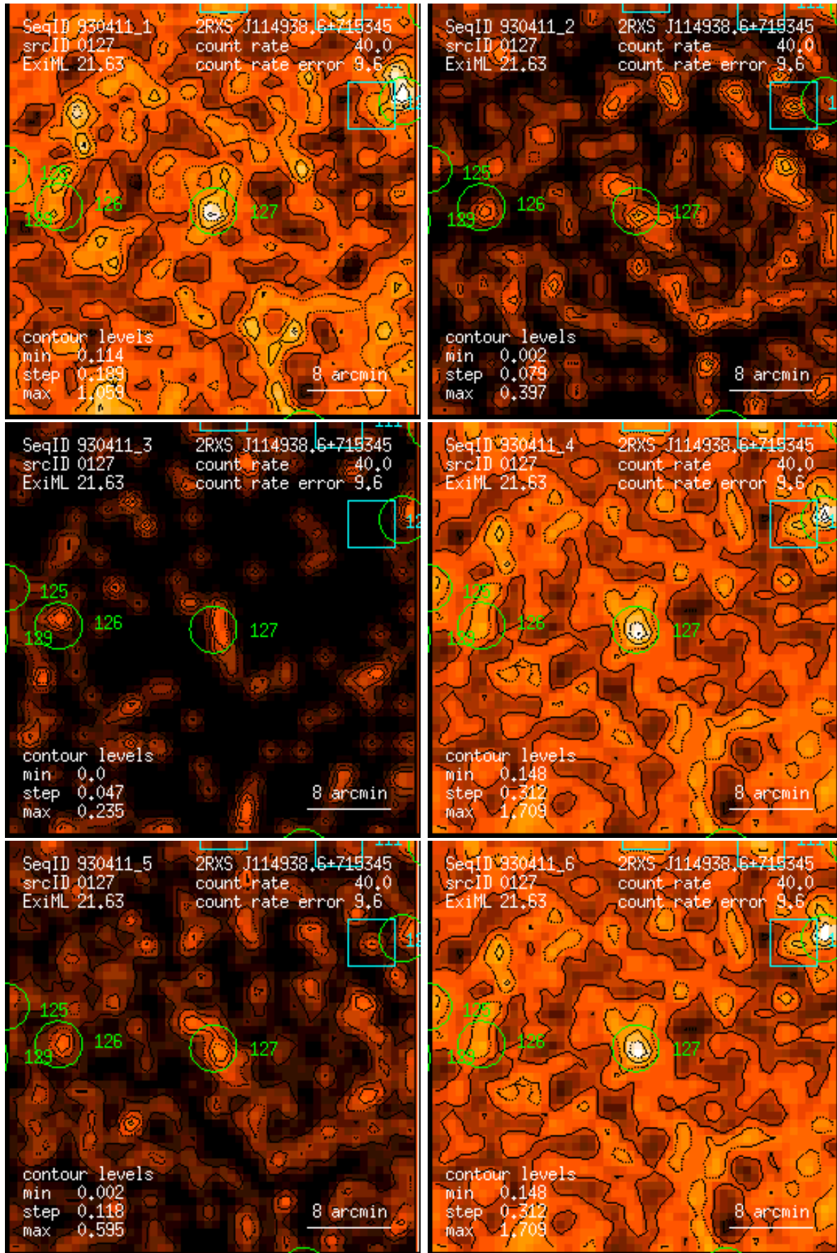
Figure 127: RASS 930411: detection 0127: band rate images, Gaussian filter: (1) PSPC channels 11 – 41, (2) 52 – 90, (3) 91 – 201, (4) 11 – 235, (5) 52 – 201, (6) 11 – 201. Broad band rates in counts/ks. Band rate contour levels in counts/ks/arcmin 2 .
