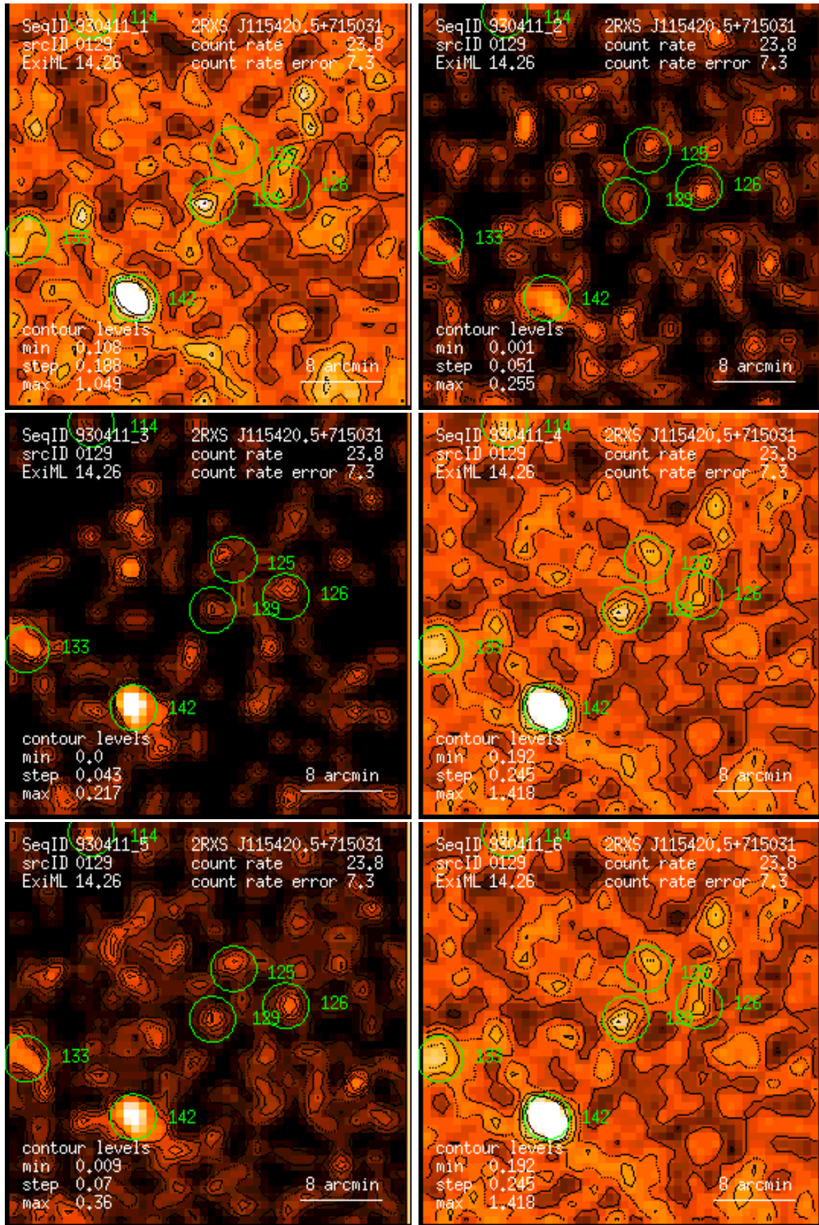
Figure 129: RASS 930411: detection 0129: band rate images, Gaussian filter: (1) PSPC channels 11 – 41, (2) 52 – 90, (3) 91 – 201, (4) 11 – 235, (5) 52 – 201, (6) 11 – 201. Broad band rates in counts/ks. Band rate contour levels in counts/ks/arcmin 2 .
