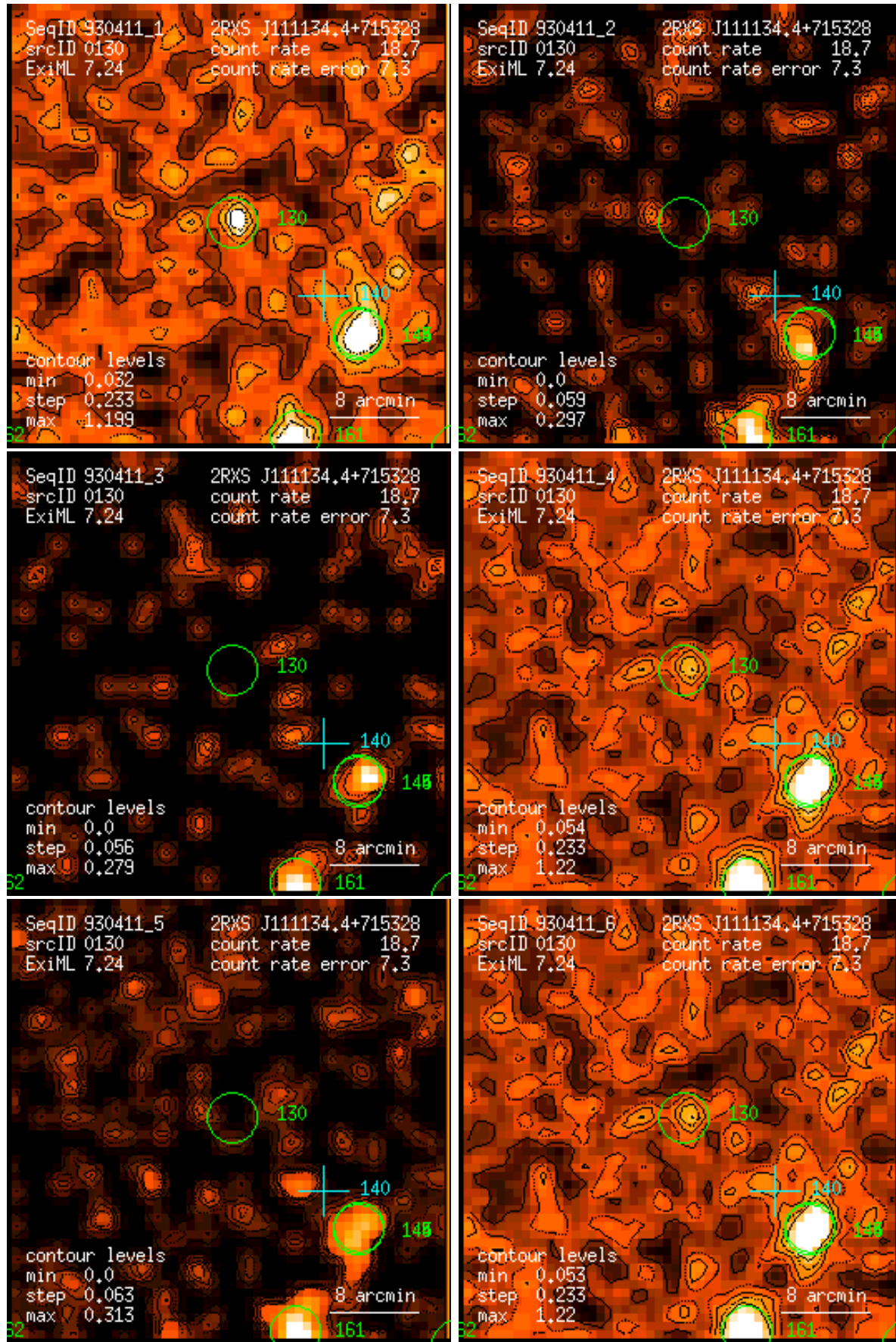
Figure 130: RASS 930411: detection 0130: band rate images, Gaussian filter: (1) PSPC channels 11 – 41, (2) 52 – 90, (3) 91 – 201, (4) 11 – 235, (5) 52 – 201, (6) 11 – 201. Broad band rates in counts/ks. Band rate contour levels in counts/ks/arcmin 2 .
