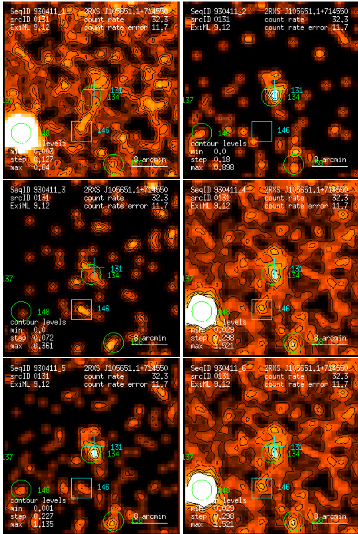
Figure 131: RASS 930411: detection 0131: band rate images, Gaussian filter: (1) PSPC channels 11 – 41, (2) 52 – 90, (3) 91 – 201, (4) 11 – 235, (5) 52 – 201, (6) 11 – 201. Broad band rates in counts/ks. Band rate contour levels in counts/ks/arcmin 2 .
