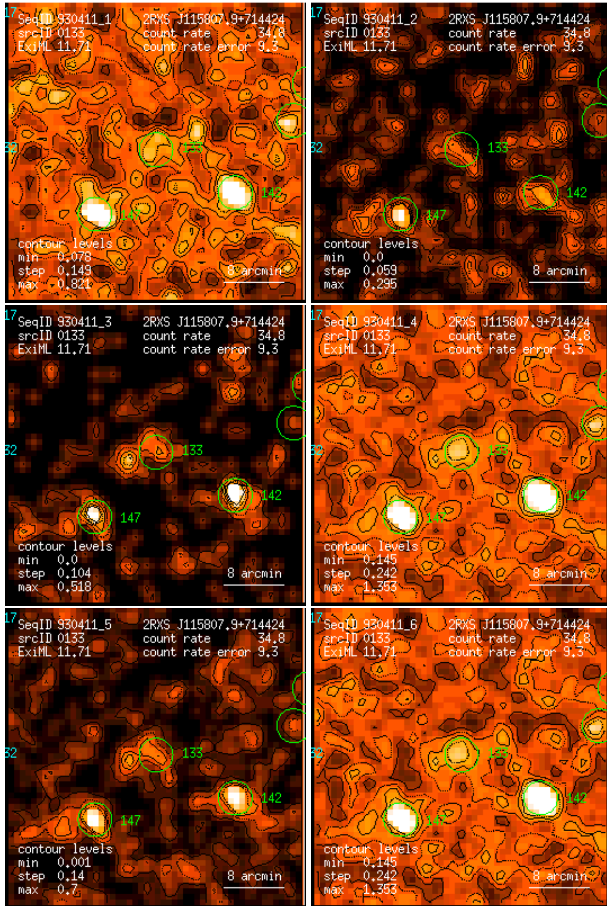
Figure 133: RASS 930411: detection 0133: band rate images, Gaussian filter: (1) PSPC channels 11 – 41, (2) 52 – 90, (3) 91 – 201, (4) 11 – 235, (5) 52 – 201, (6) 11 – 201. Broad band rates in counts/ks. Band rate contour levels in counts/ks/arcmin 2 .
