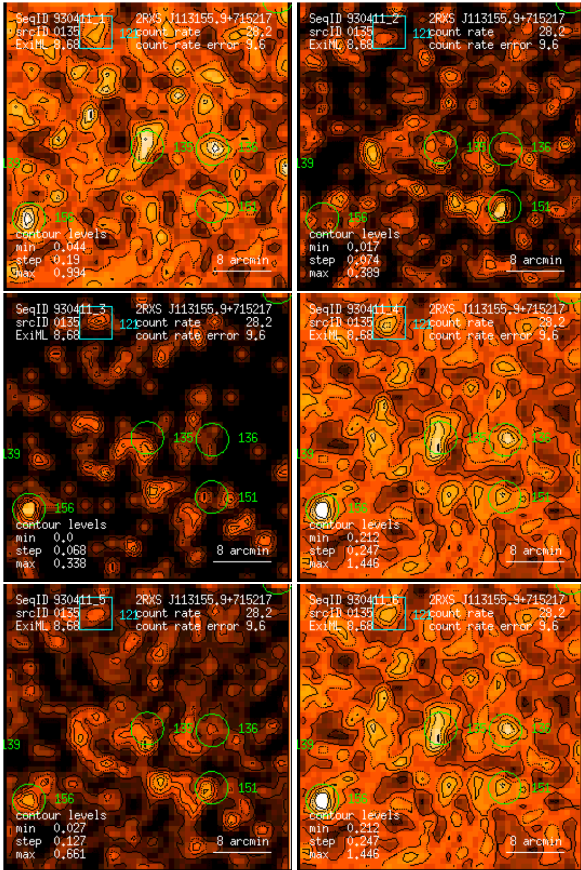
Figure 135: RASS 930411: detection 0135: band rate images, Gaussian filter: (1) PSPC channels 11 – 41, (2) 52 – 90, (3) 91 – 201, (4) 11 – 235, (5) 52 – 201, (6) 11 – 201. Broad band rates in counts/ks. Band rate contour levels in counts/ks/arcmin 2 .
