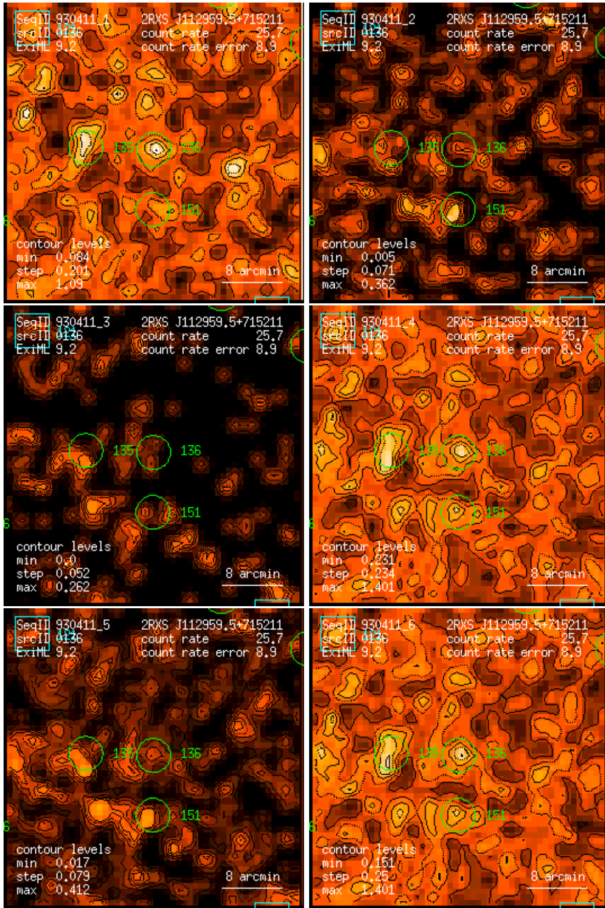
Figure 136: RASS 930411: detection 0136: band rate images, Gaussian filter: (1) PSPC channels 11 – 41, (2) 52 – 90, (3) 91 – 201, (4) 11 – 235, (5) 52 – 201, (6) 11 – 201. Broad band rates in counts/ks. Band rate contour levels in counts/ks/arcmin 2 .
