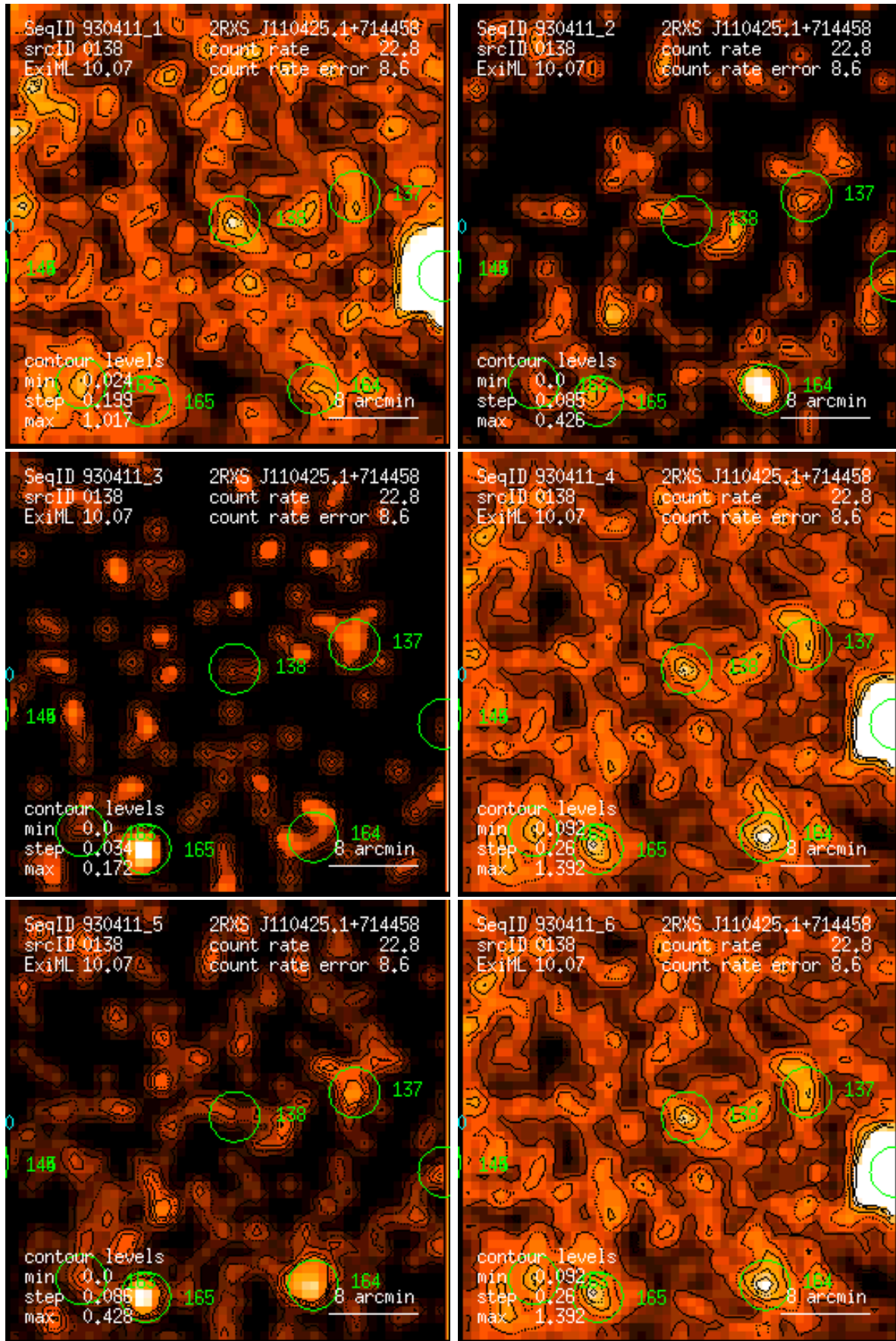
Figure 138: RASS 930411: detection 0138: band rate images, Gaussian filter: (1) PSPC channels 11 – 41, (2) 52 – 90, (3) 91 – 201, (4) 11 – 235, (5) 52 – 201, (6) 11 – 201. Broad band rates in counts/ks. Band rate contour levels in counts/ks/arcmin 2 .
