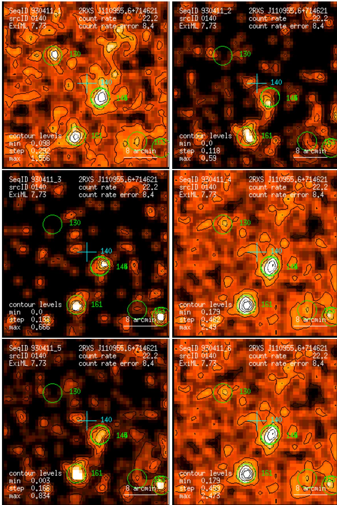
Figure 140: RASS 930411: detection 0140: band rate images, Gaussian filter: (1) PSPC channels 11 – 41, (2) 52 – 90, (3) 91 – 201, (4) 11 – 235, (5) 52 – 201, (6) 11 – 201. Broad band rates in counts/ks. Band rate contour levels in counts/ks/arcmin 2 .
