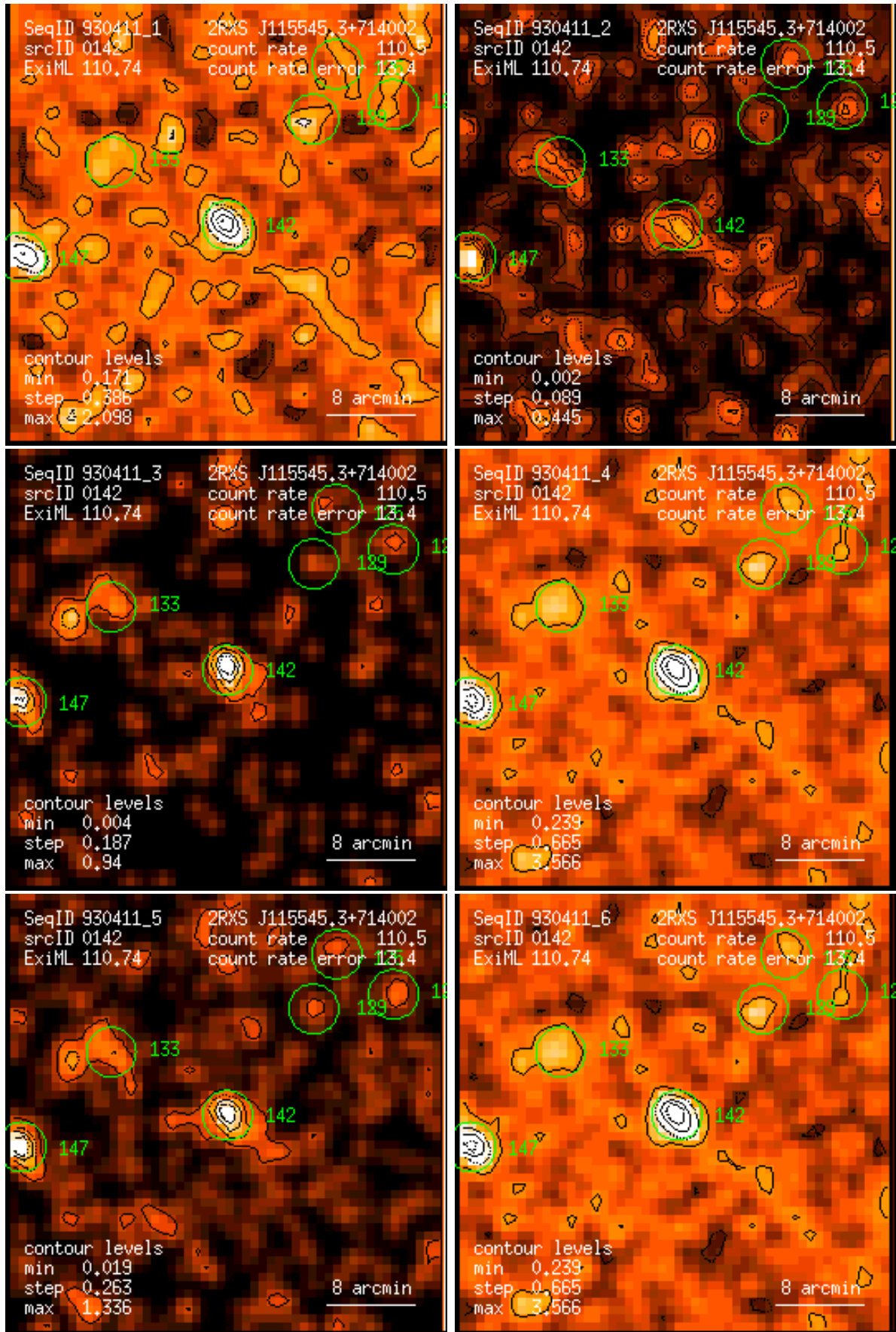
Figure 142: RASS 930411: detection 0142: band rate images, Gaussian filter: (1) PSPC channels 11 – 41, (2) 52 – 90, (3) 91 – 201, (4) 11 – 235, (5) 52 – 201, (6) 11 – 201. Broad band rates in counts/ks. Band rate contour levels in counts/ks/arcmin 2 .
