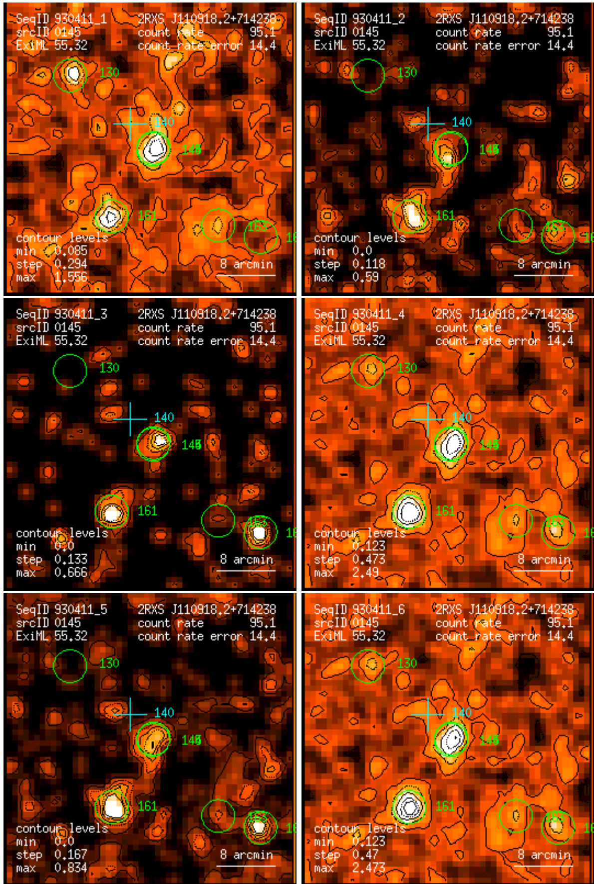
Figure 145: RASS 930411: detection 0145: band rate images, Gaussian filter: (1) PSPC channels 11 – 41, (2) 52 – 90, (3) 91 – 201, (4) 11 – 235, (5) 52 – 201, (6) 11 – 201. Broad band rates in counts/ks. Band rate contour levels in counts/ks/arcmin 2 .
