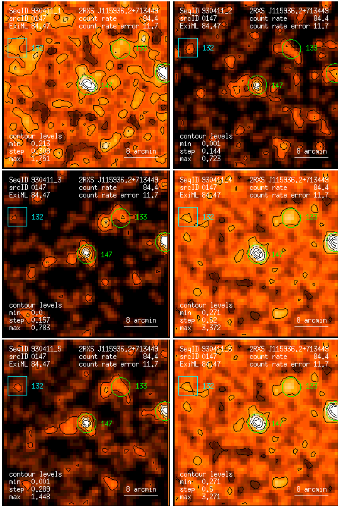
Figure 147: RASS 930411: detection 0147: band rate images, Gaussian filter: (1) PSPC channels 11 – 41, (2) 52 – 90, (3) 91 – 201, (4) 11 – 235, (5) 52 – 201, (6) 11 – 201. Broad band rates in counts/ks. Band rate contour levels in counts/ks/arcmin 2 .
