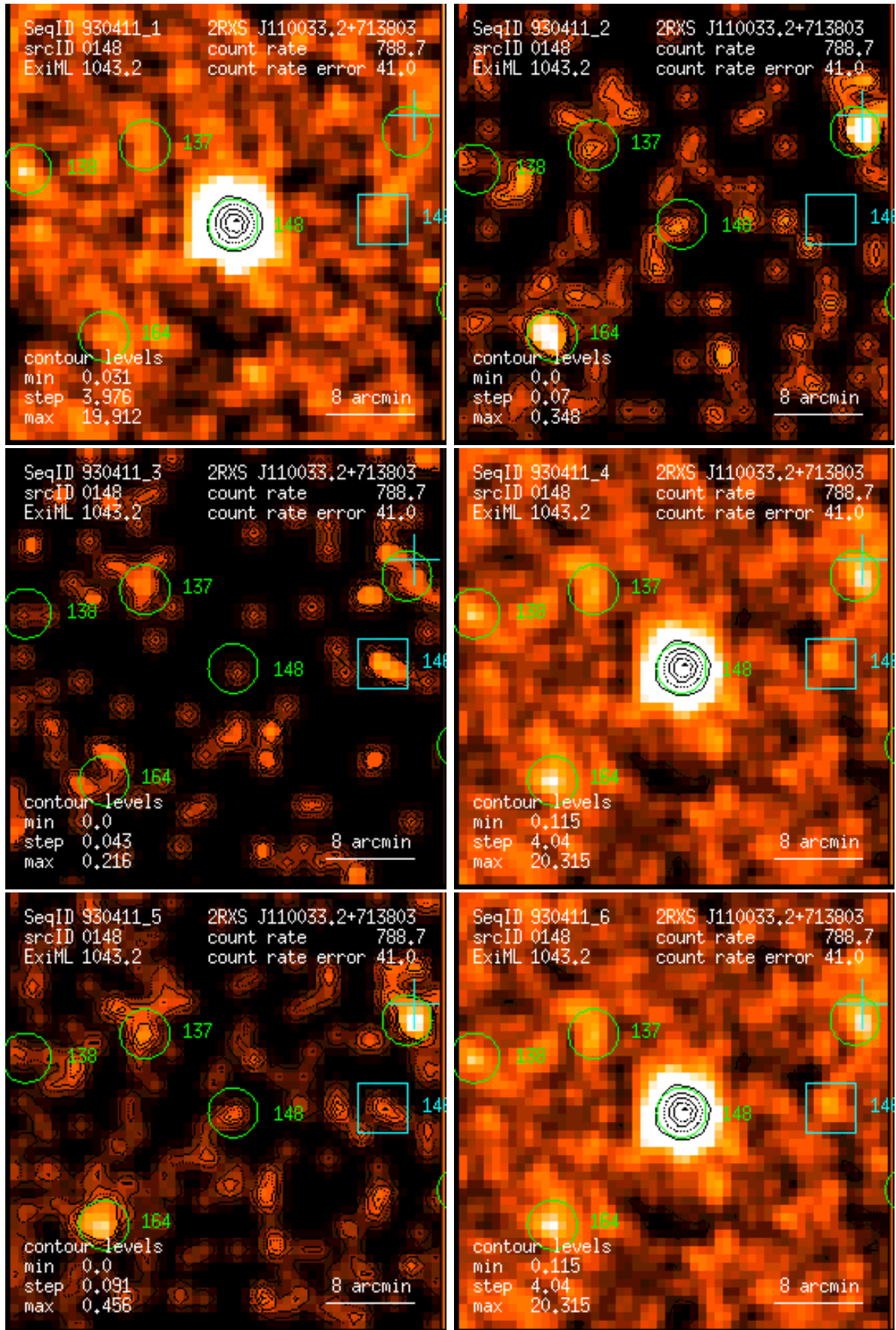
Figure 148: RASS 930411: detection 0148: band rate images, Gaussian filter: (1) PSPC channels 11 – 41, (2) 52 – 90, (3) 91 – 201, (4) 11 – 235, (5) 52 – 201, (6) 11 – 201. Broad band rates in counts/ks. Band rate contour levels in counts/ks/arcmin 2 .
