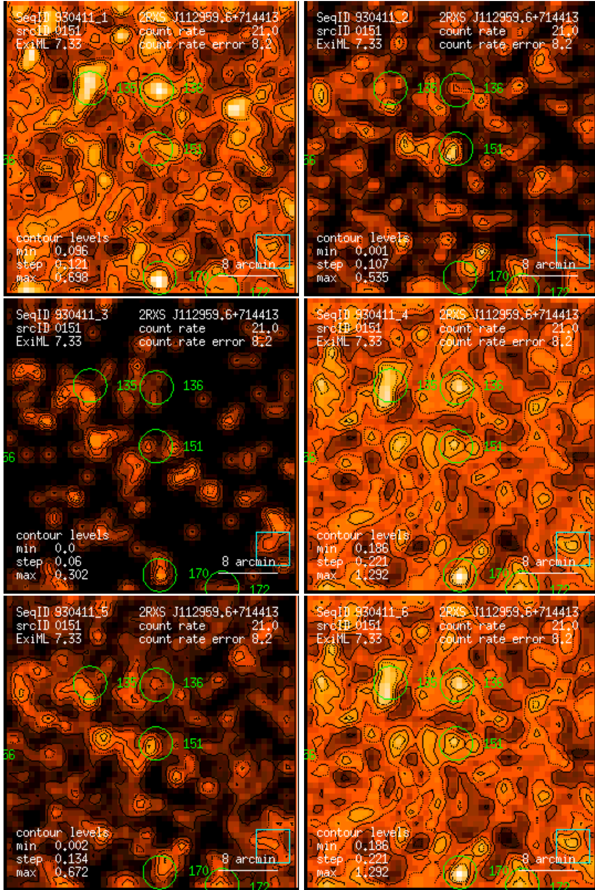
Figure 151: RASS 930411: detection 0151: band rate images, Gaussian filter: (1) PSPC channels 11 – 41, (2) 52 – 90, (3) 91 – 201, (4) 11 – 235, (5) 52 – 201, (6) 11 – 201. Broad band rates in counts/ks. Band rate contour levels in counts/ks/arcmin 2 .
