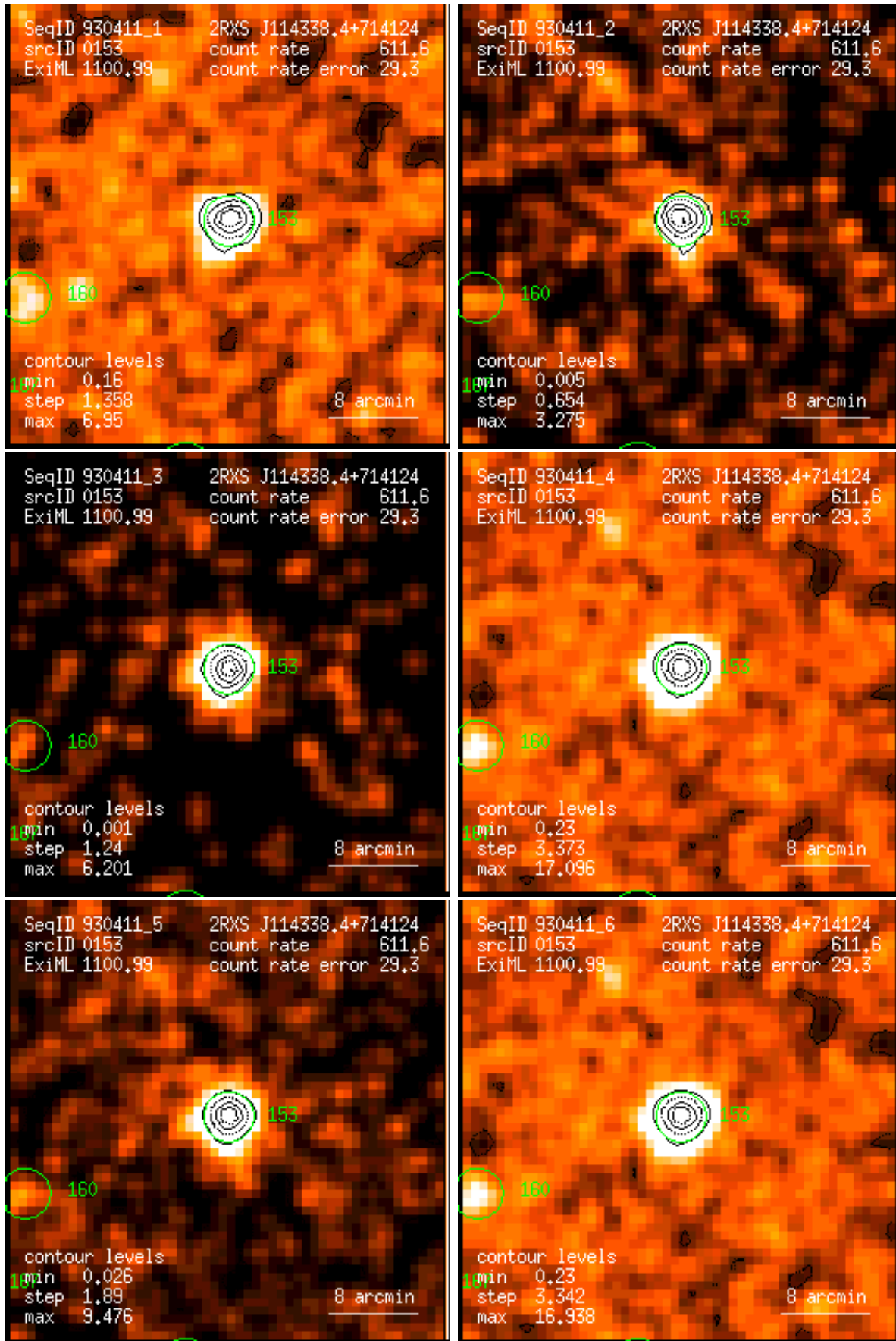
Figure 153: RASS 930411: detection 0153: band rate images, Gaussian filter: (1) PSPC channels 11 – 41, (2) 52 – 90, (3) 91 – 201, (4) 11 – 235, (5) 52 – 201, (6) 11 – 201. Broad band rates in counts/ks. Band rate contour levels in counts/ks/arcmin 2 .
