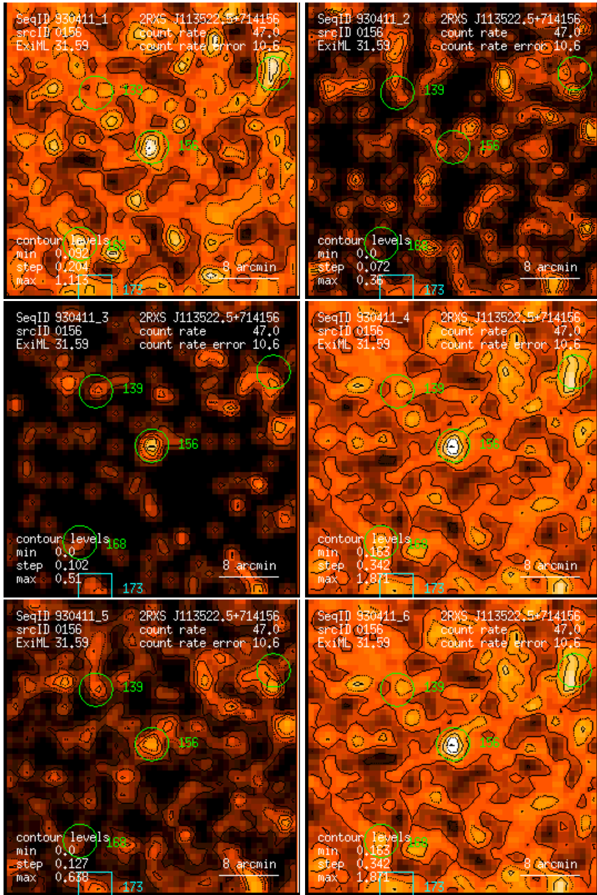
Figure 156: RASS 930411: detection 0156: band rate images, Gaussian filter: (1) PSPC channels 11 – 41, (2) 52 – 90, (3) 91 – 201, (4) 11 – 235, (5) 52 – 201, (6) 11 – 201. Broad band rates in counts/ks. Band rate contour levels in counts/ks/arcmin 2 .
