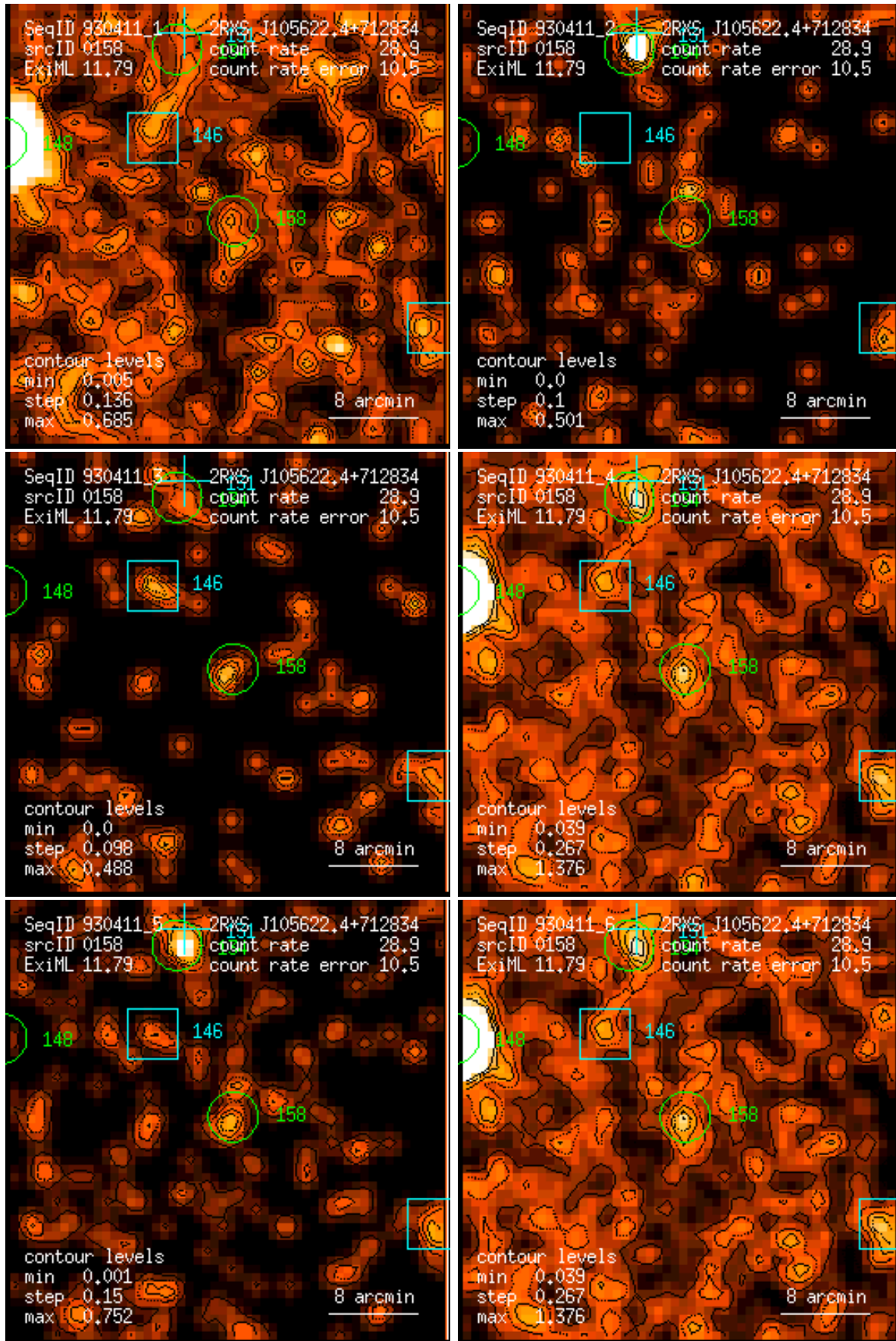
Figure 158: RASS 930411: detection 0158: band rate images, Gaussian filter: (1) PSPC channels 11 – 41, (2) 52 – 90, (3) 91 – 201, (4) 11 – 235, (5) 52 – 201, (6) 11 – 201. Broad band rates in counts/ks. Band rate contour levels in counts/ks/arcmin 2 .
