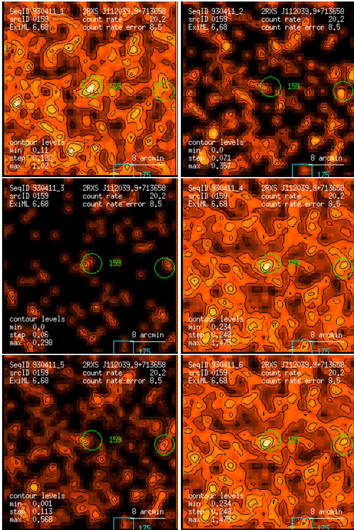
Figure 159: RASS 930411: detection 0159: band rate images, Gaussian filter: (1) PSPC channels 11 – 41, (2) 52 – 90, (3) 91 – 201, (4) 11 – 235, (5) 52 – 201, (6) 11 – 201. Broad band rates in counts/ks. Band rate contour levels in counts/ks/arcmin 2 .
