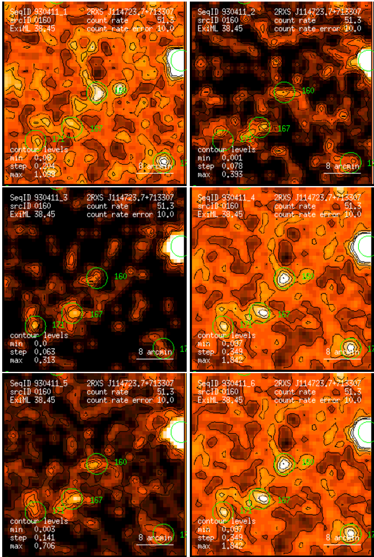
Figure 160: RASS 930411: detection 0160: band rate images, Gaussian filter: (1) PSPC channels 11 – 41, (2) 52 – 90, (3) 91 – 201, (4) 11 – 235, (5) 52 – 201, (6) 11 – 201. Broad band rates in counts/ks. Band rate contour levels in counts/ks/arcmin 2 .
