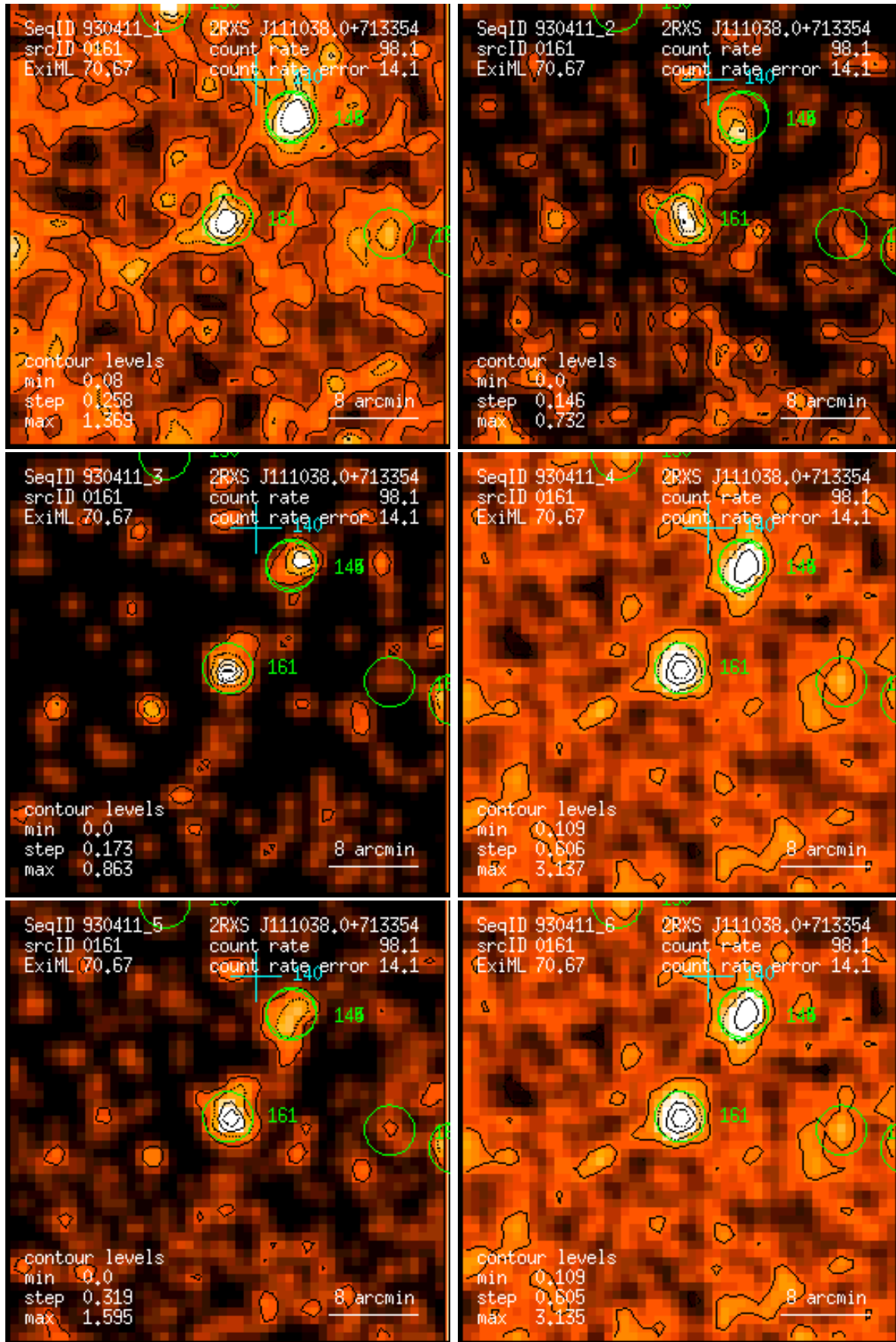
Figure 161: RASS 930411: detection 0161: band rate images, Gaussian filter: (1) PSPC channels 11 – 41, (2) 52 – 90, (3) 91 – 201, (4) 11 – 235, (5) 52 – 201, (6) 11 – 201. Broad band rates in counts/ks. Band rate contour levels in counts/ks/arcmin 2 .
