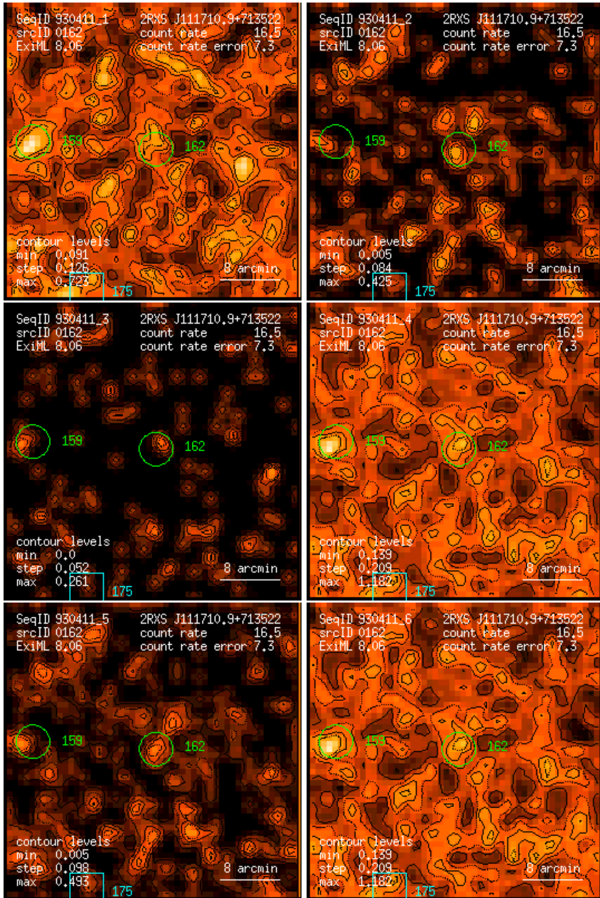
Figure 162: RASS 930411: detection 0162: band rate images, Gaussian filter: (1) PSPC channels 11 – 41, (2) 52 – 90, (3) 91 – 201, (4) 11 – 235, (5) 52 – 201, (6) 11 – 201. Broad band rates in counts/ks. Band rate contour levels in counts/ks/arcmin 2 .
