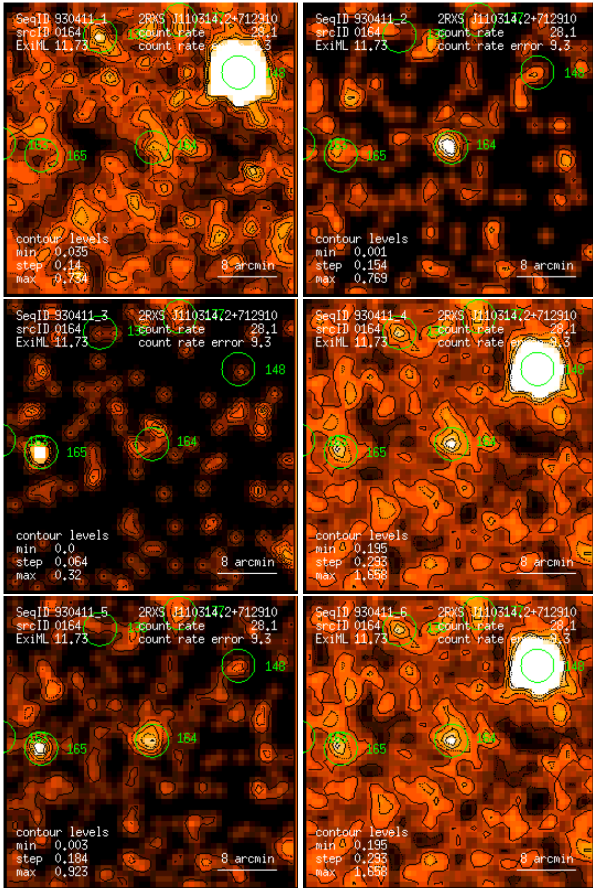
Figure 164: RASS 930411: detection 0164: band rate images, Gaussian filter: (1) PSPC channels 11 – 41, (2) 52 – 90, (3) 91 – 201, (4) 11 – 235, (5) 52 – 201, (6) 11 – 201. Broad band rates in counts/ks. Band rate contour levels in counts/ks/arcmin 2 .
