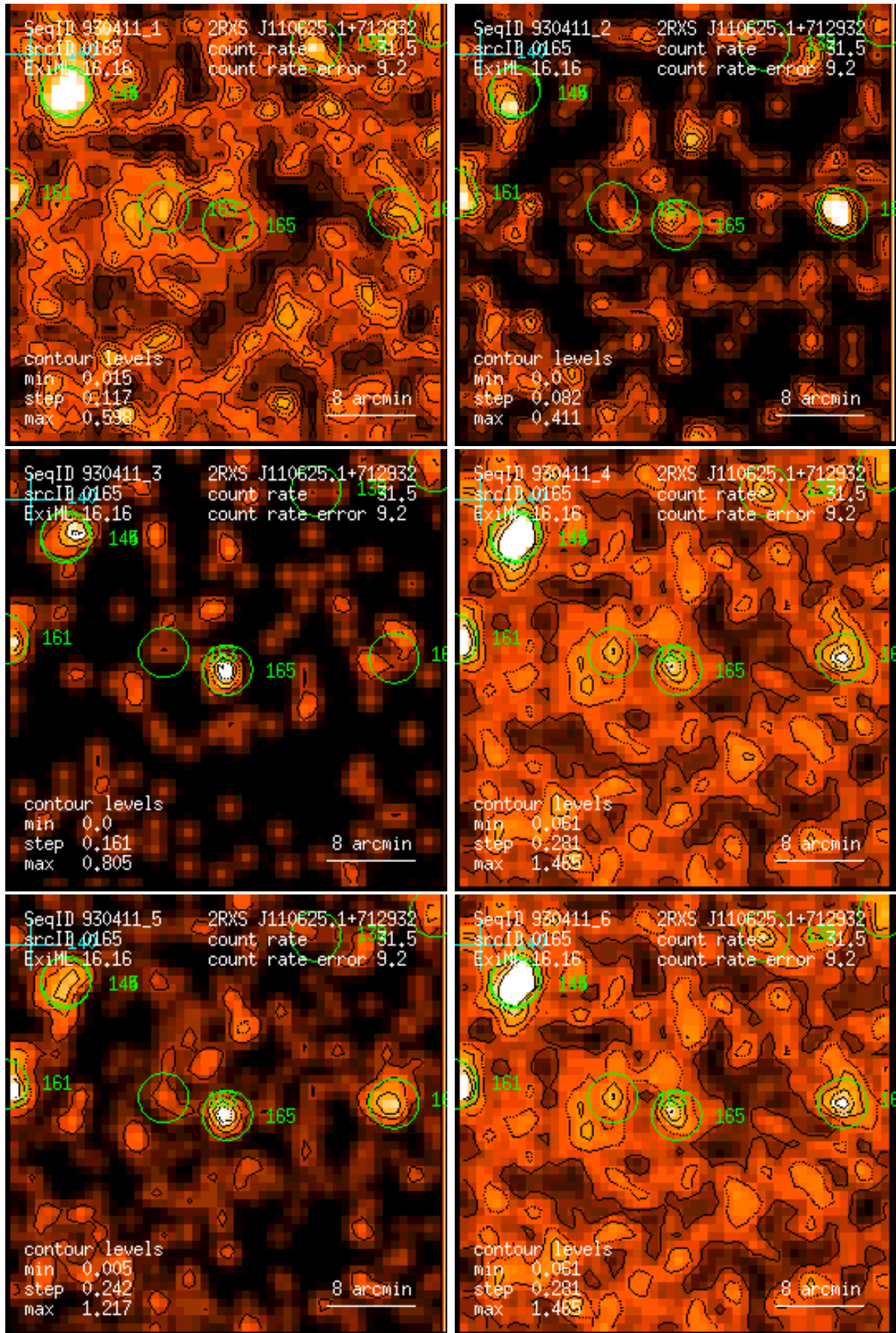
Figure 165: RASS 930411: detection 0165: band rate images, Gaussian filter: (1) PSPC channels 11 – 41, (2) 52 – 90, (3) 91 – 201, (4) 11 – 235, (5) 52 – 201, (6) 11 – 201. Broad band rates in counts/ks. Band rate contour levels in counts/ks/arcmin 2 .
