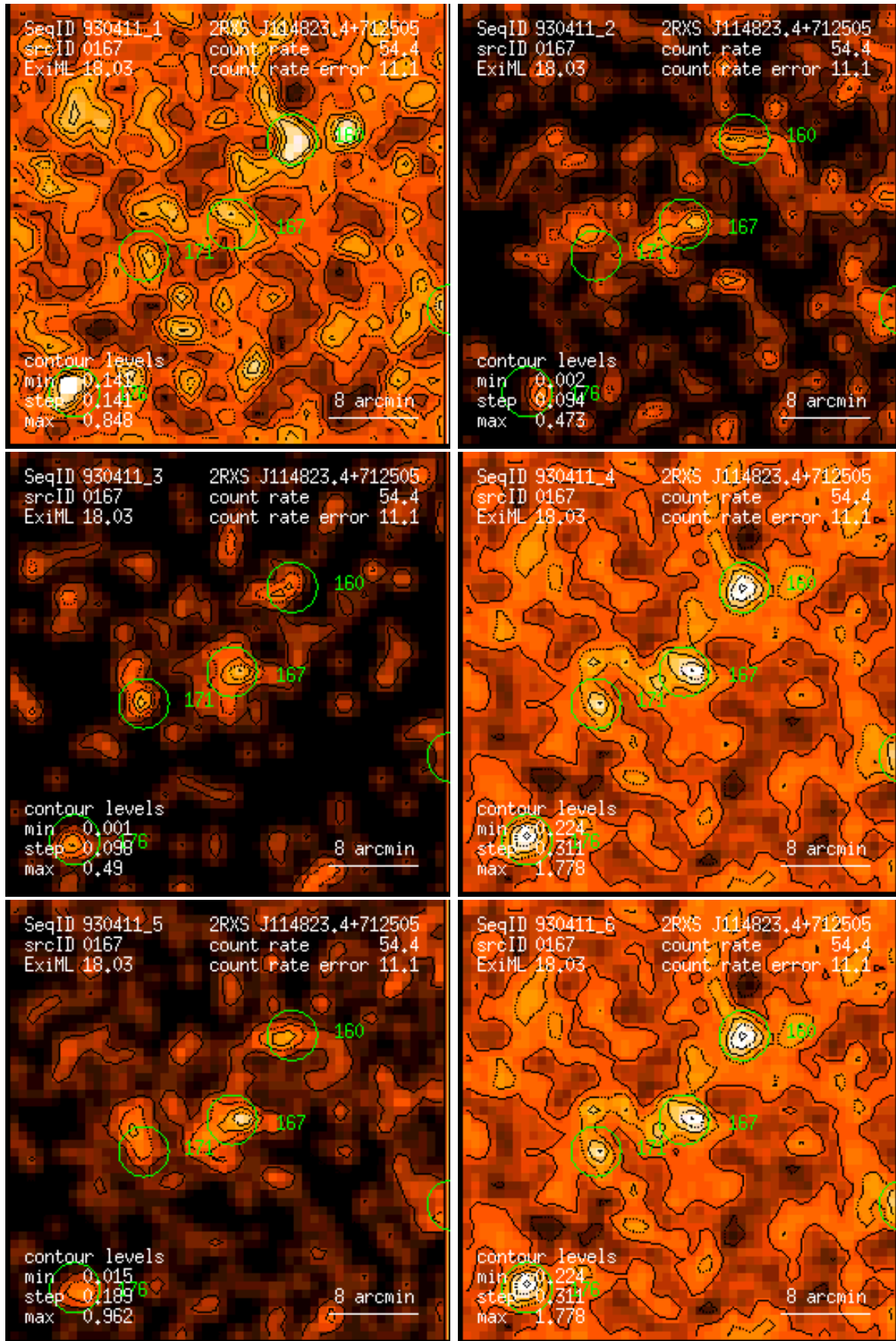
Figure 167: RASS 930411: detection 0167: band rate images, Gaussian filter: (1) PSPC channels 11 – 41, (2) 52 – 90, (3) 91 – 201, (4) 11 – 235, (5) 52 – 201, (6) 11 – 201. Broad band rates in counts/ks. Band rate contour levels in counts/ks/arcmin 2 .
