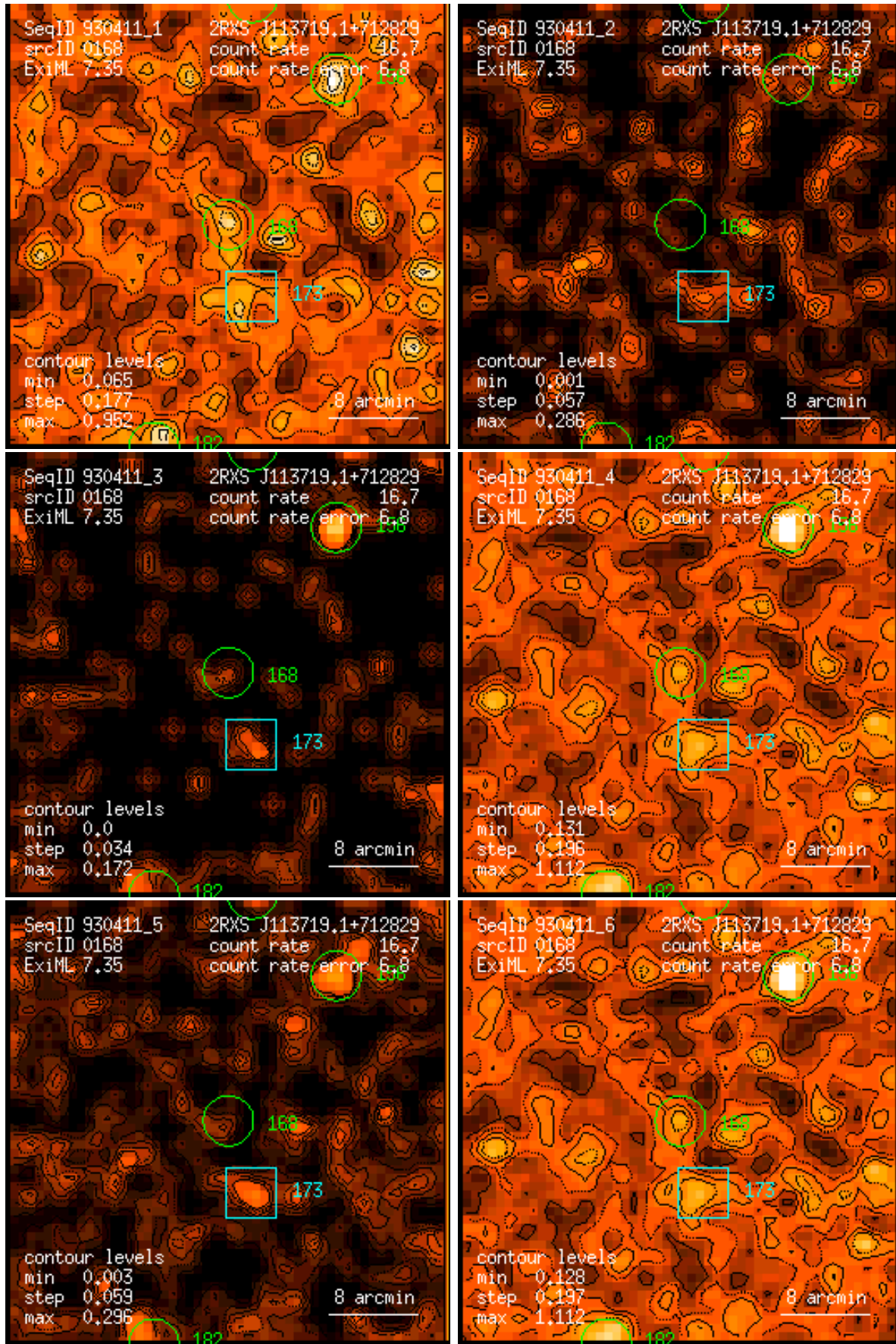
Figure 168: RASS 930411: detection 0168: band rate images, Gaussian filter: (1) PSPC channels 11 – 41, (2) 52 – 90, (3) 91 – 201, (4) 11 – 235, (5) 52 – 201, (6) 11 – 201. Broad band rates in counts/ks. Band rate contour levels in counts/ks/arcmin 2 .
