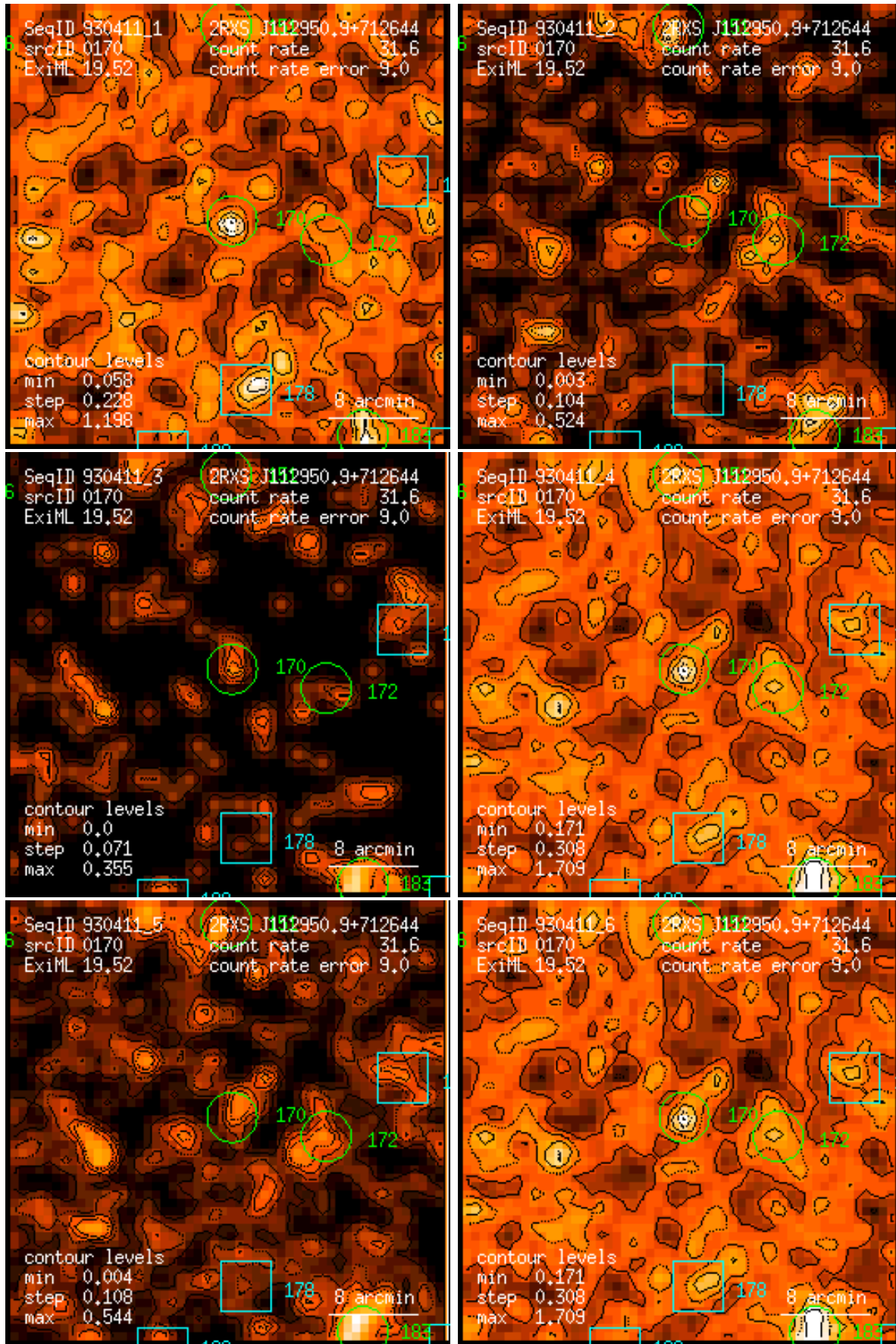
Figure 170: RASS 930411: detection 0170: band rate images, Gaussian filter: (1) PSPC channels 11 – 41, (2) 52 – 90, (3) 91 – 201, (4) 11 – 235, (5) 52 – 201, (6) 11 – 201. Broad band rates in counts/ks. Band rate contour levels in counts/ks/arcmin 2 .
