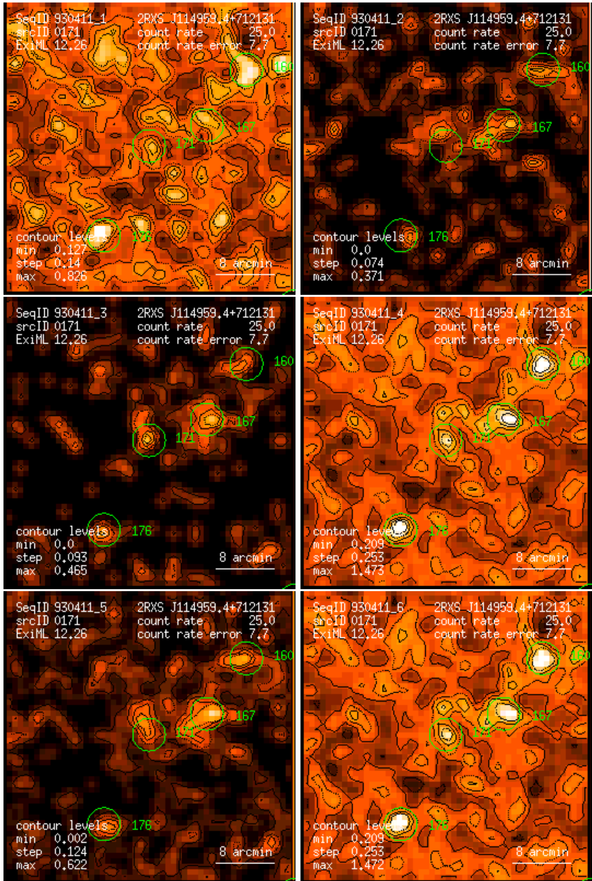
Figure 171: RASS 930411: detection 0171: band rate images, Gaussian filter: (1) PSPC channels 11 – 41, (2) 52 – 90, (3) 91 – 201, (4) 11 – 235, (5) 52 – 201, (6) 11 – 201. Broad band rates in counts/ks. Band rate contour levels in counts/ks/arcmin 2 .
