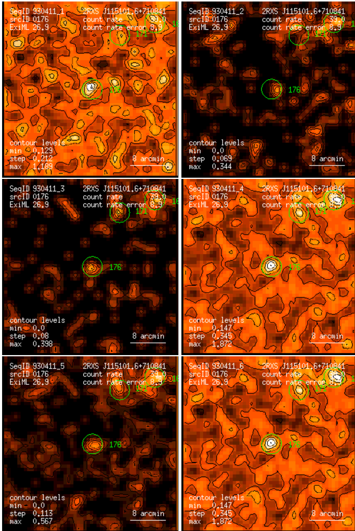
Figure 176: RASS 930411: detection 0176: band rate images, Gaussian filter: (1) PSPC channels 11 – 41, (2) 52 – 90, (3) 91 – 201, (4) 11 – 235, (5) 52 – 201, (6) 11 – 201. Broad band rates in counts/ks. Band rate contour levels in counts/ks/arcmin 2 .
