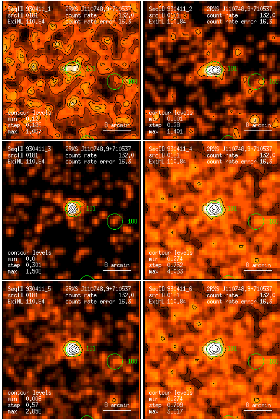
Figure 181: RASS 930411: detection 0181: band rate images, Gaussian filter: (1) PSPC channels 11 – 41, (2) 52 – 90, (3) 91 – 201, (4) 11 – 235, (5) 52 – 201, (6) 11 – 201. Broad band rates in counts/ks. Band rate contour levels in counts/ks/arcmin 2 .
