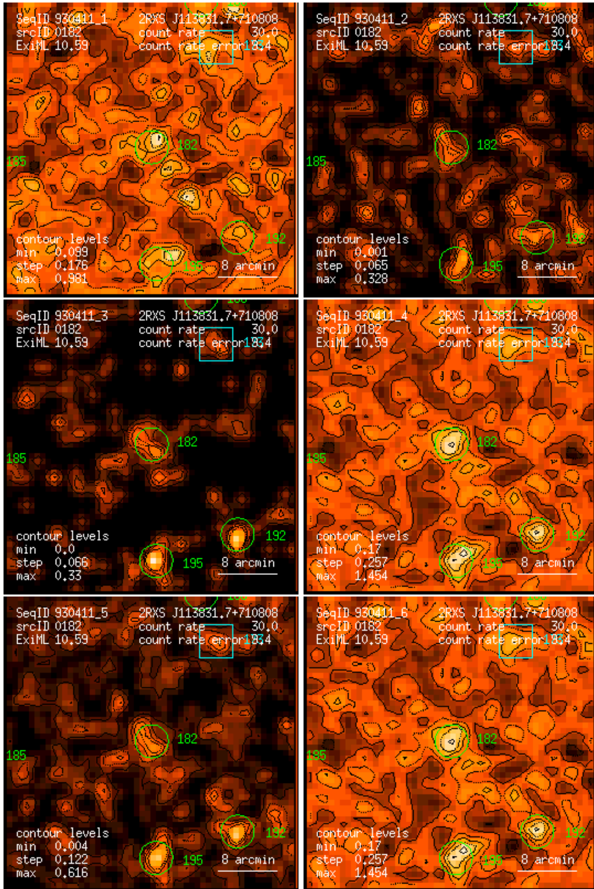
Figure 182: RASS 930411: detection 0182: band rate images, Gaussian filter: (1) PSPC channels 11 – 41, (2) 52 – 90, (3) 91 – 201, (4) 11 – 235, (5) 52 – 201, (6) 11 – 201. Broad band rates in counts/ks. Band rate contour levels in counts/ks/arcmin 2 .
