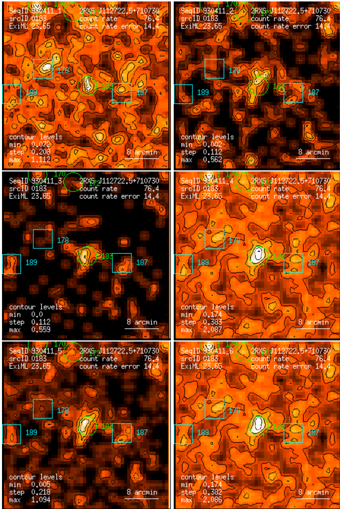
Figure 183: RASS 930411: detection 0183: band rate images, Gaussian filter: (1) PSPC channels 11 – 41, (2) 52 – 90, (3) 91 – 201, (4) 11 – 235, (5) 52 – 201, (6) 11 – 201. Broad band rates in counts/ks. Band rate contour levels in counts/ks/arcmin 2 .
