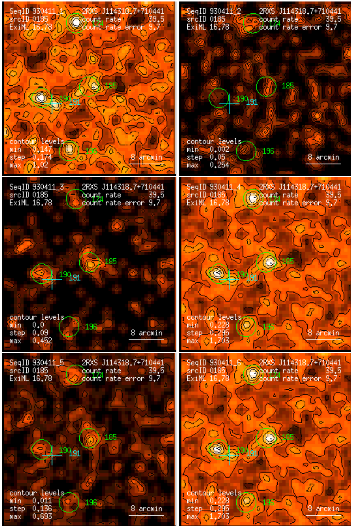
Figure 185: RASS 930411: detection 0185: band rate images, Gaussian filter: (1) PSPPC channels 11 – 41, (2) 52 – 90, (3) 91 – 201, (4) 11 – 235, (5) 52 – 201, (6) 11 – 201. Broad band rates in counts/ks. Band rate contour levels in counts/ks/arcmin 2 .
