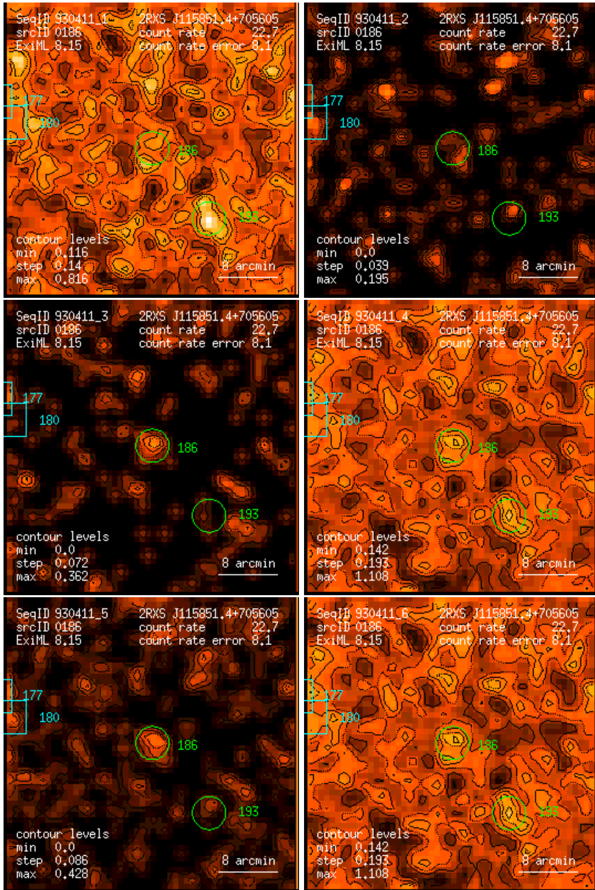
Figure 186: RASS 930411: detection 0186: band rate images, Gaussian filter: (1) PSPC channels 11 – 41, (2) 52 – 90, (3) 91 – 201, (4) 11 – 235, (5) 52 – 201, (6) 11 – 201. Broad band rates in counts/ks. Band rate contour levels in counts/ks/arcmin 2 .
