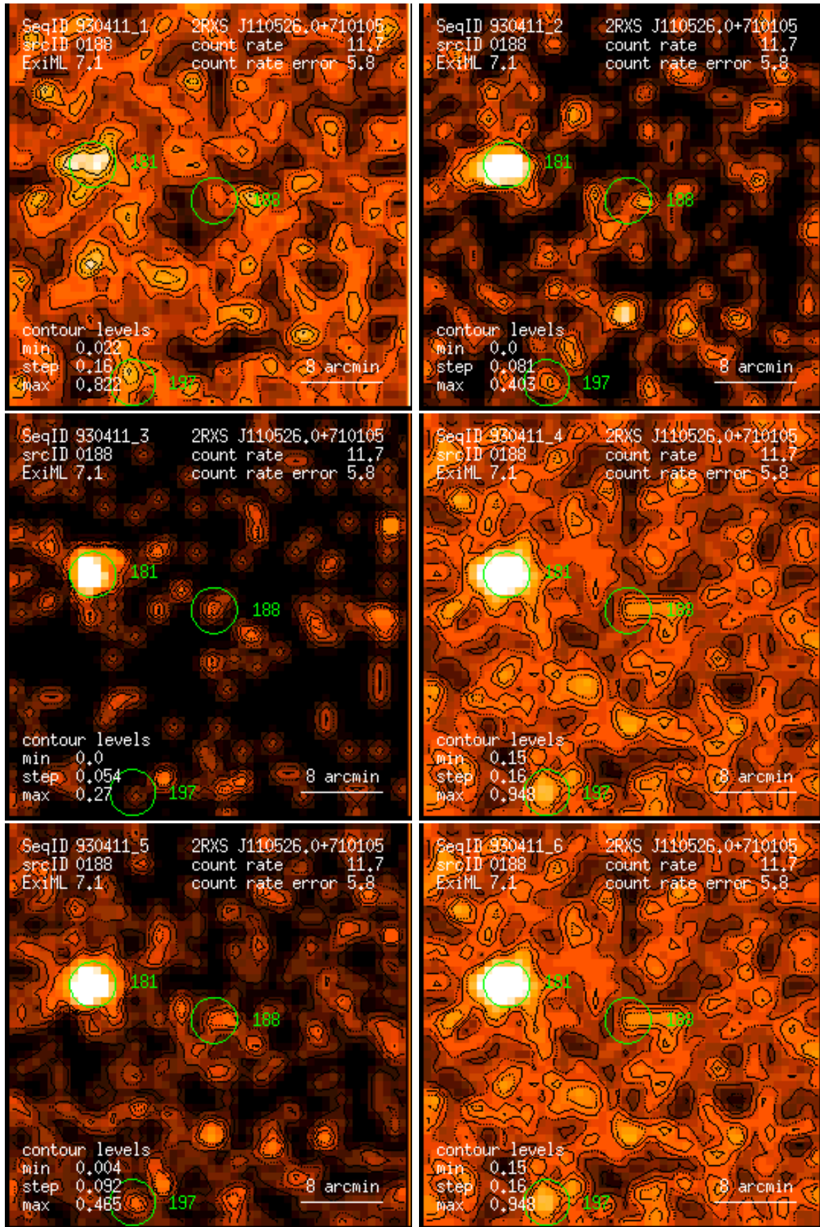
Figure 188: RASS 930411: detection 0188: band rate images, Gaussian filter: (1) PSPC channels 11 – 41, (2) 52 – 90, (3) 91 – 201, (4) 11 – 235, (5) 52 – 201, (6) 11 – 201. Broad band rates in counts/ks. Band rate contour levels in counts/ks/arcmin 2 .
