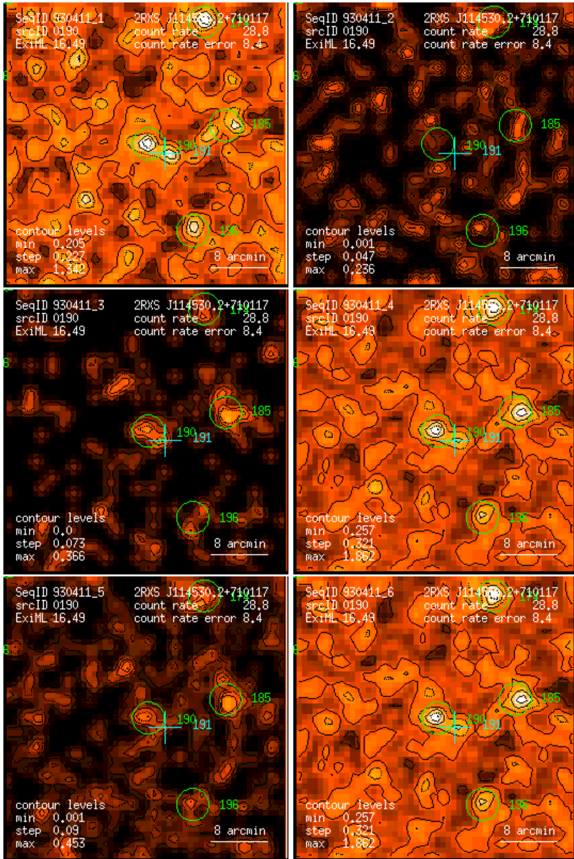
Figure 190: RASS 930411: detection 0190: band rate images, Gaussian filter: (1) PSPC channels 11 – 41, (2) 52 – 90, (3) 91 – 201, (4) 11 – 235, (5) 52 – 201, (6) 11 – 201. Broad band rates in counts/ks. Band rate contour levels in counts/ks/arcmin 2 .
