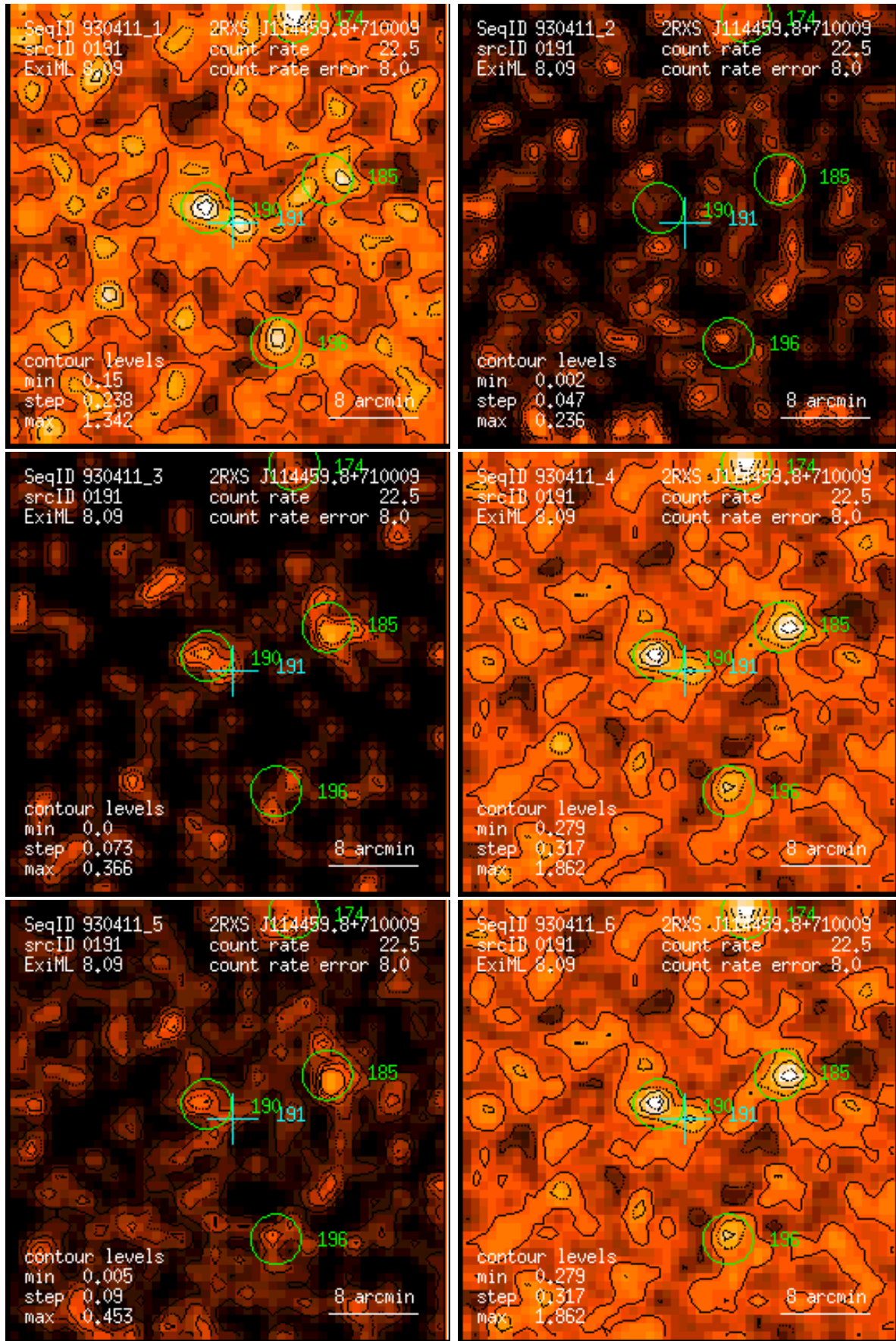
Figure 191: RASS 930411: detection 0191: band rate images, Gaussian filter: (1) PSPC channels 11 – 41, (2) 52 – 90, (3) 91 – 201, (4) 11 – 235, (5) 52 – 201, (6) 11 – 201. Broad band rates in counts/ks. Band rate contour levels in counts/ks/arcmin 2 .
