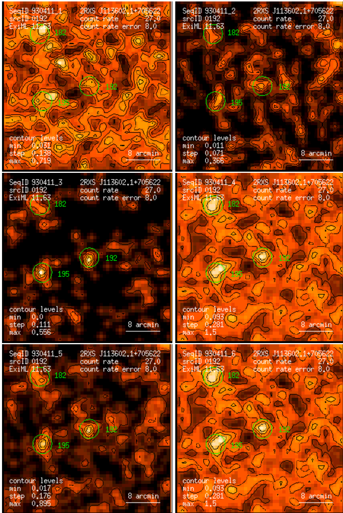
Figure 192: RASS 930411: detection 0192: band rate images, Gaussian filter: (1) PSPC channels 11 – 41, (2) 52 – 90, (3) 91 – 201, (4) 11 – 235, (5) 52 – 201, (6) 11 – 201. Broad band rates in counts/ks. Band rate contour levels in counts/ks/arcmin 2 .
