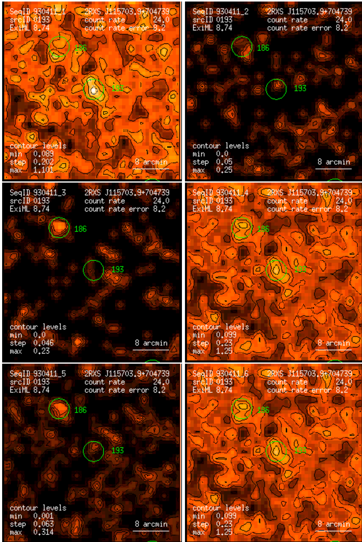
Figure 193: RASS 930411: detection 0193: band rate images, Gaussian filter: (1) PSPC channels 11 – 41, (2) 52 – 90, (3) 91 – 201, (4) 11 – 235, (5) 52 – 201, (6) 11 – 201. Broad band rates in counts/ks. Band rate contour levels in counts/ks/arcmin 2 .
