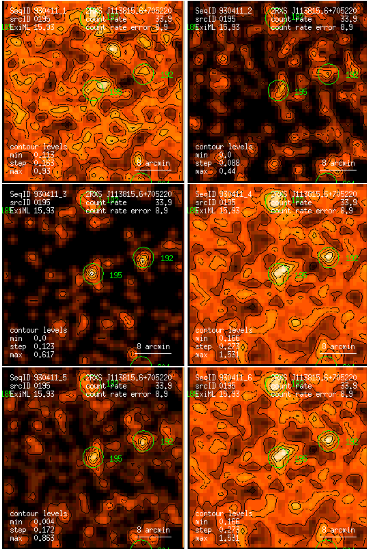
Figure 195: RASS 930411: detection 0195: band rate images, Gaussian filter: (1) PSPC channels 11 – 41, (2) 52 – 90, (3) 91 – 201, (4) 11 – 235, (5) 52 – 201, (6) 11 – 201. Broad band rates in counts/ks. Band rate contour levels in counts/ks/arcmin 2 .
